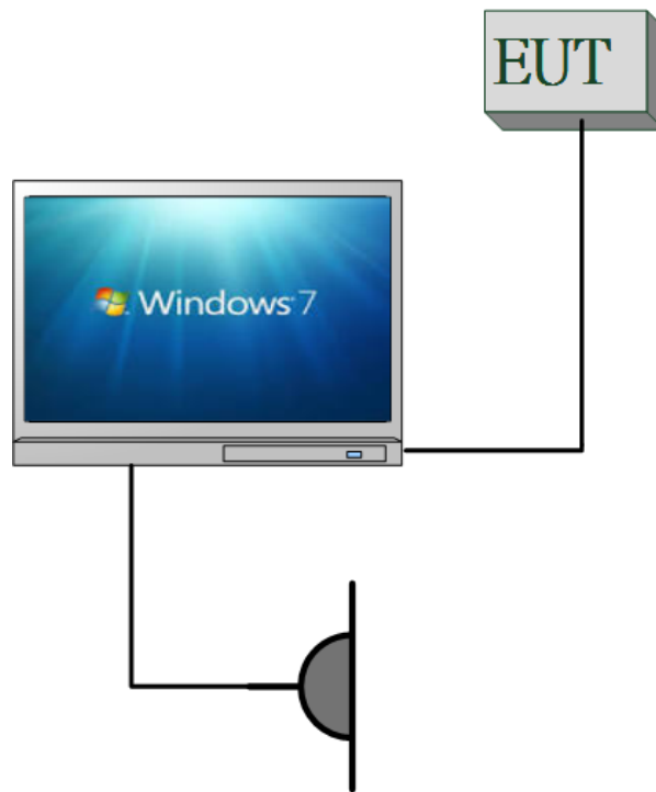
Fig. 2-2 AC Power Line Conducted Emission Configuration
