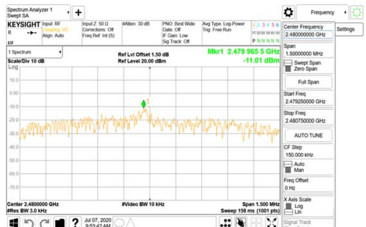
Power Density_BLE_2M_HighCH39-2480
