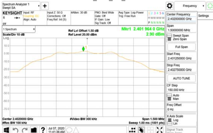
Reference Level_BLE_1M_LowCH00-2402
