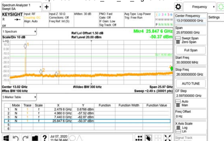
Spurious Emission_BLE_1M_HighCH39-2480
