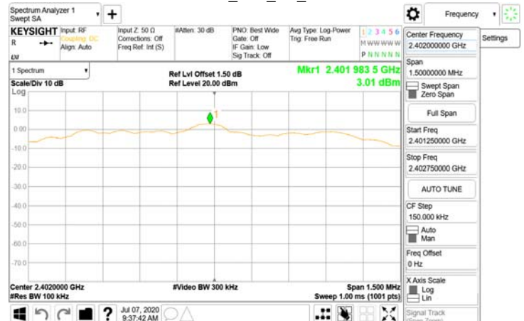
Reference Level_BLE_2M_LowCH00-2402
