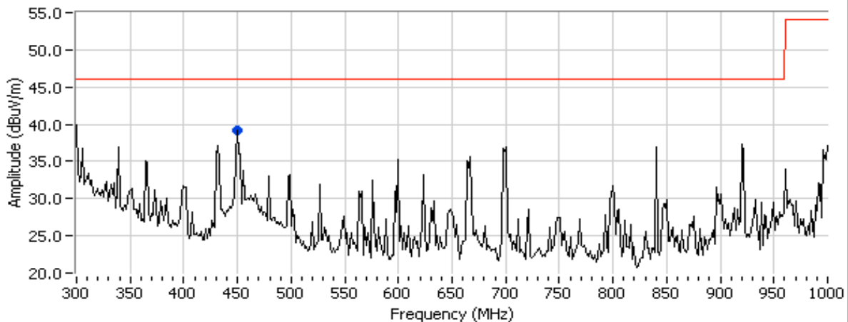
Channel @ 2437MHz
