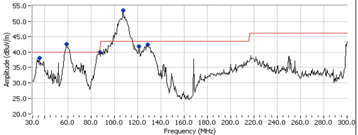
Channel @ 2437MHz
