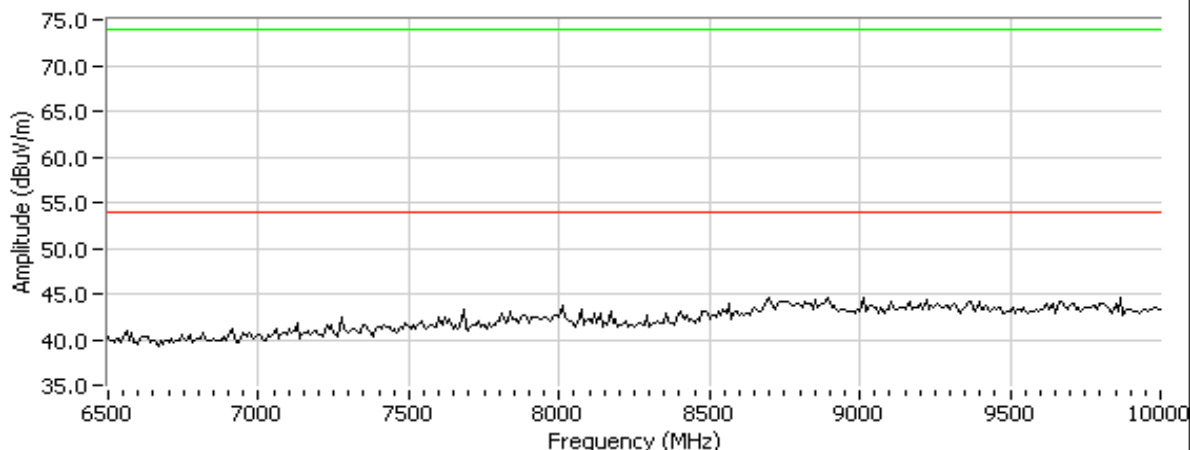
5755MHz, Chain A, 802.11n-40
