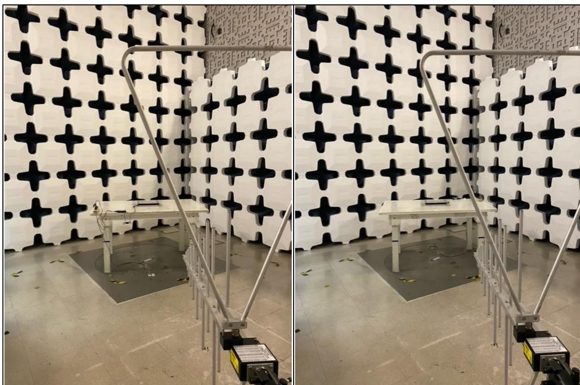
Radiated Emission Test (Below 1GHz)
