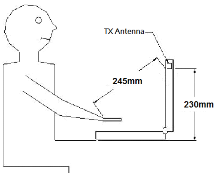
Fig.9 Antenna location of laptop mode - End of Report -
