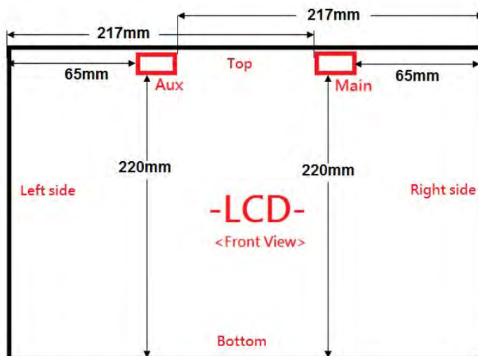
Fig.7 Antenna location of tablet mode (front view)
