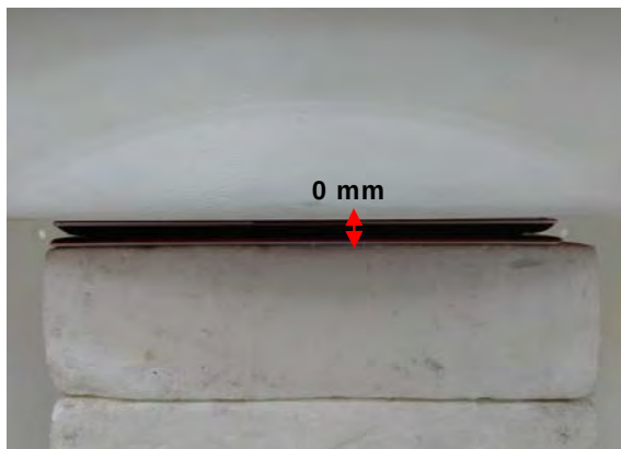
Fig.3 EUT Back side_Tablet mode to flat phantom
