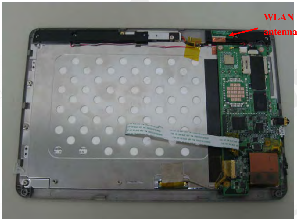
Fig.10 Antenna position of EUT
