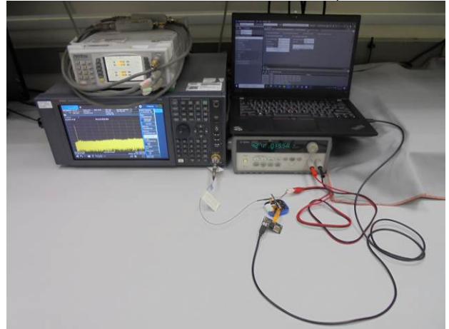
FCC_15_247_BLE_Conducted_setup
