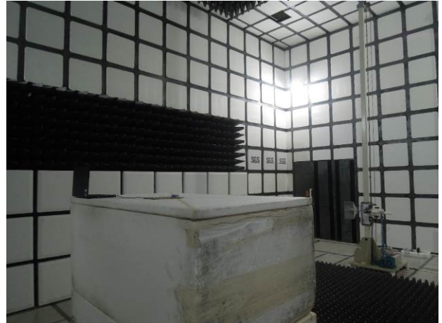
FCC_15_247_BLE_Radiated_Setup_2nd Source
