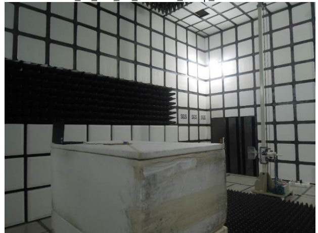
FCC_15_247_BT_Radiated_Setup_2nd Source
