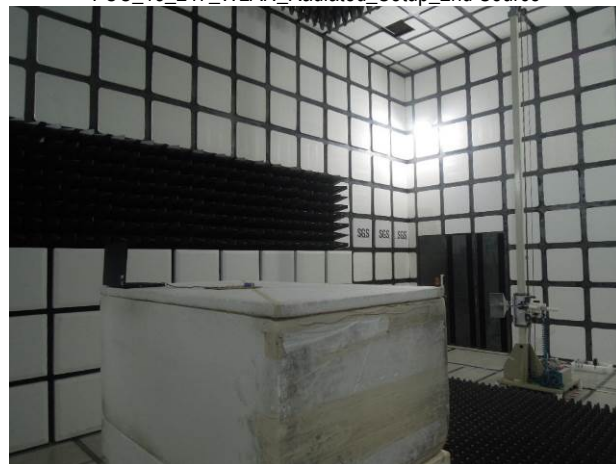
FCC_15_247_WLAN_Radiated_Setup_2nd Source
