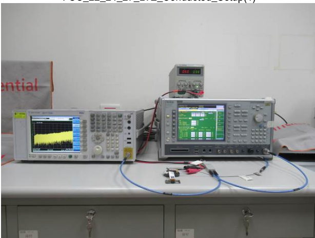
FCC 22 24 27_LTE_Conducted_Setup(1)
