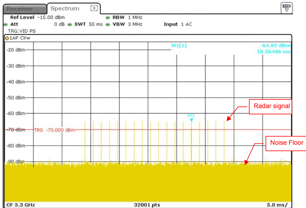
Radar Signal 0
