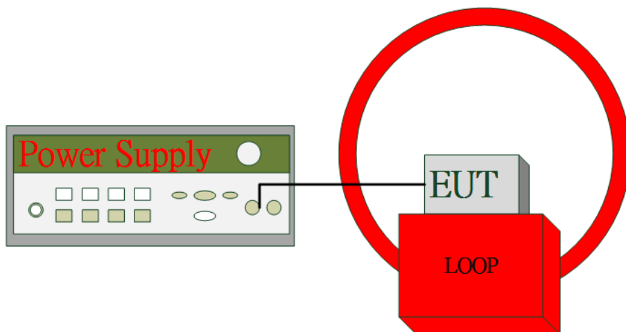
Fig. 2-1 Conducted Emission
