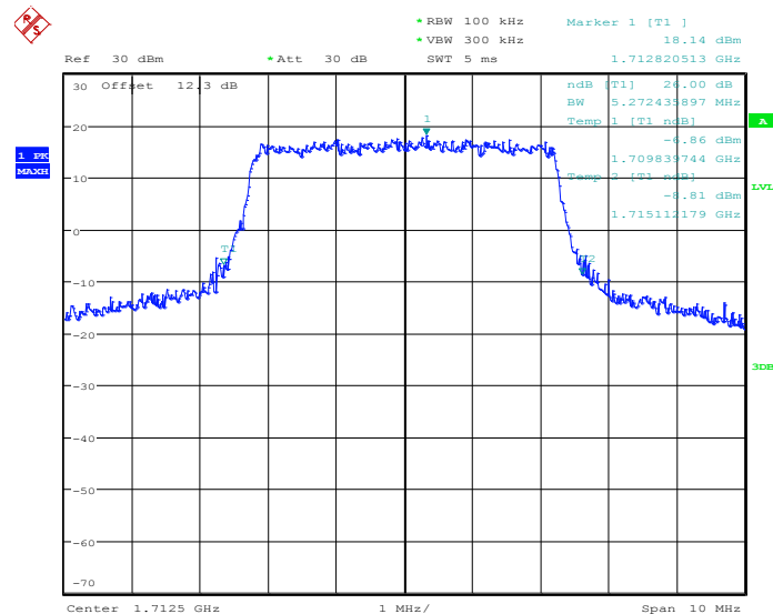
26dB Bandwidth Plot on Channel 19975
