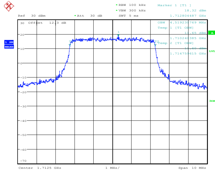
99% Occupied Bandwidth Plot on Channel 19975
