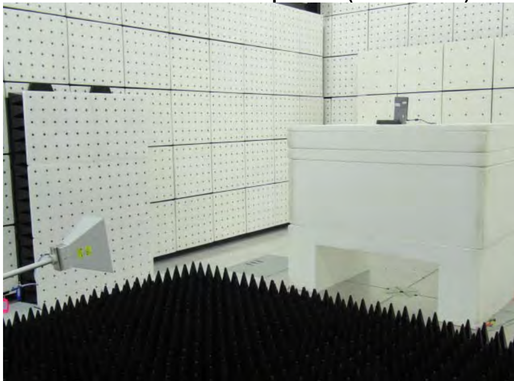
Radiated Emission Set up Photo (Front View)
