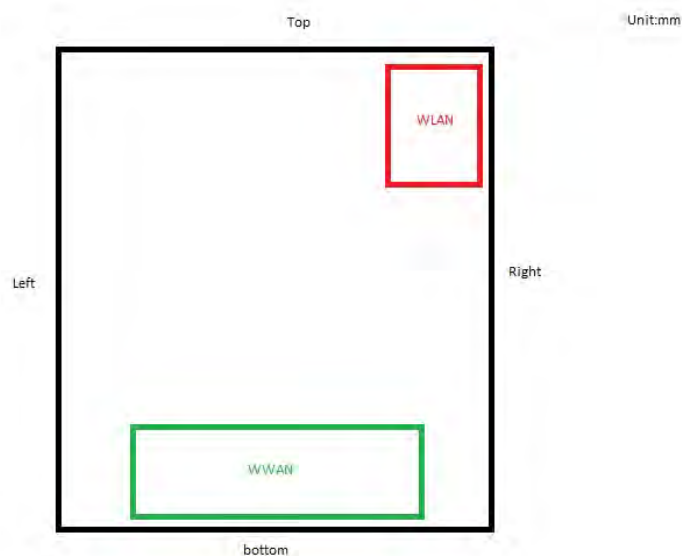
Fig.18 Antenna position of EUT
