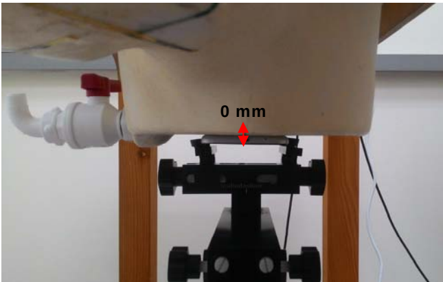
Fig.7 EUT Back side to flat phantom
