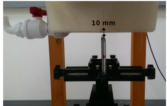
Fig.12 EUT right to flat phantom
