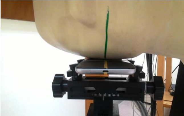
Fig.3 Right Head Section / Cheek-Touch Position
