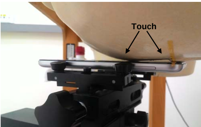
Fig.5 Left Head Section / Cheek-Touch Position
