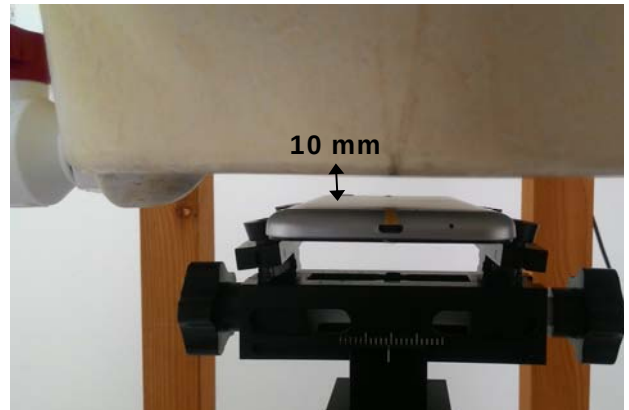
Fig.9 EUT back side to flat phantom
