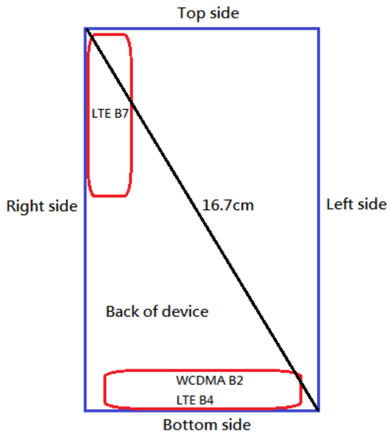
Fig.16 Antenna position of EUT
