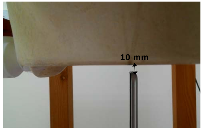
Fig.10 EUT bottom side to flat phantom
