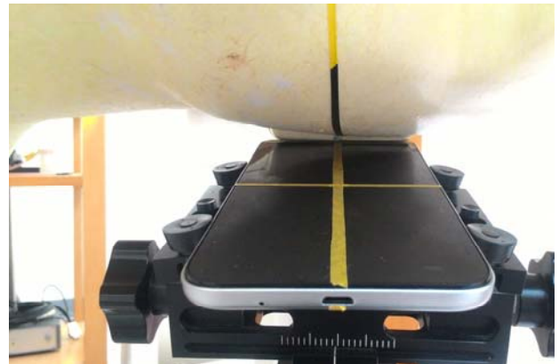
Fig.6 Left Head Section / Ear-Tilt Position(15°)
