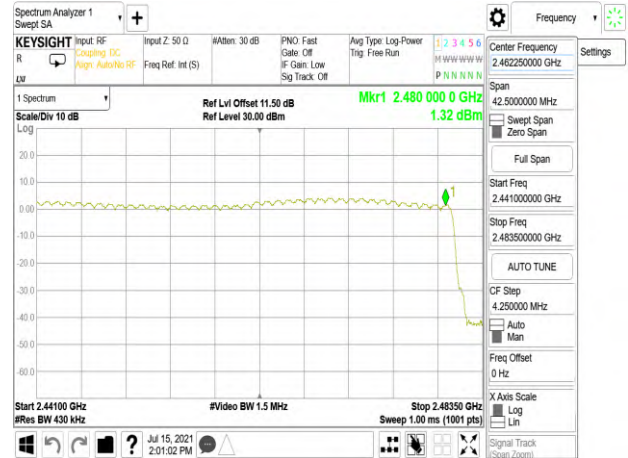
4DQPSK_2M_DH5_2441-2480
