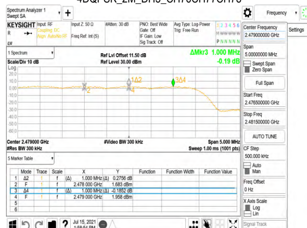
4DQPSK_2M_DH5_CH76CH77CH78
