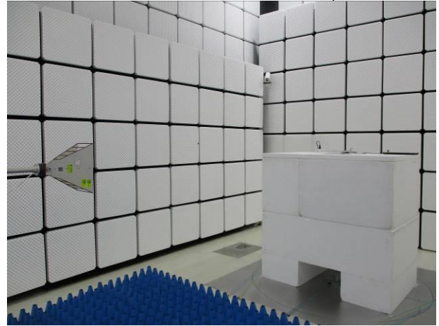
FCC_15_247_WLAN_Radiated_Setup
