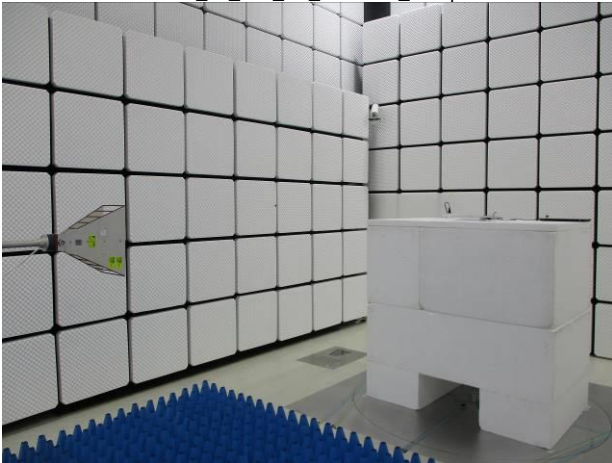
FCC_15_247_BT_Radiated_Setup
