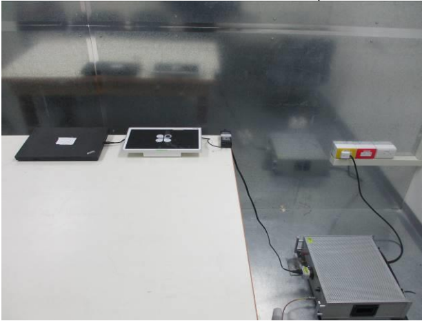
FCC_15_247_BT_Conduction_Setup
