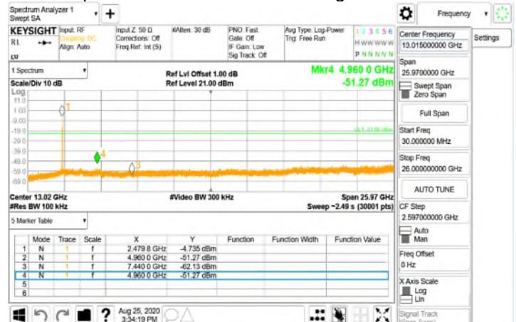
Spurious Emission_BLE_2M_HighCH39-2480
