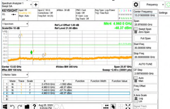
Spurious Emission_BLE_1M_HighCH39-2480
