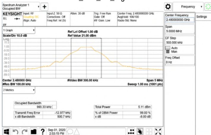
OBW 6dB_BLE_1M_HighCH39-2480
