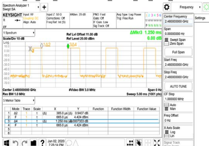
FCC_15_247_BT\Dwell Time_GFSK_1M_DH1_2480MHz
