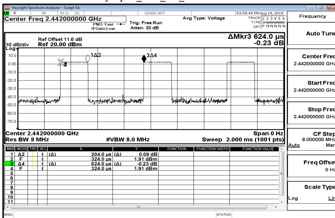
Duty Cycle_BLE_2M_MidCH20-2442
