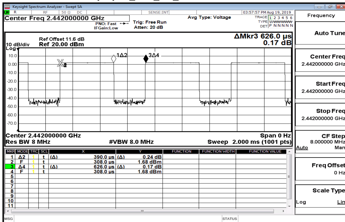
Duty Cycle_BLE_1M_MidCH20-2442
