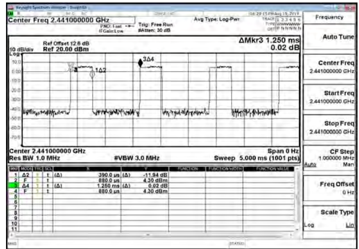
Dwell Time_π/4DQPSK_2M_DH3_2441MHz
