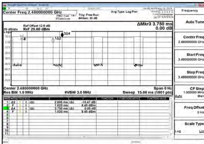
Dwell Time_GFSK_1M_DH5_2480MHz
