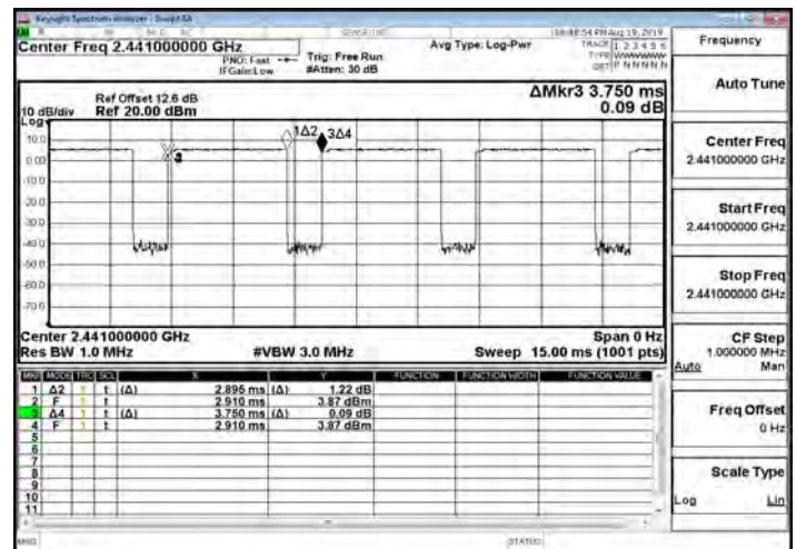
Dwell Time_π/4DQPSK_2M_DH5_2441MHz
