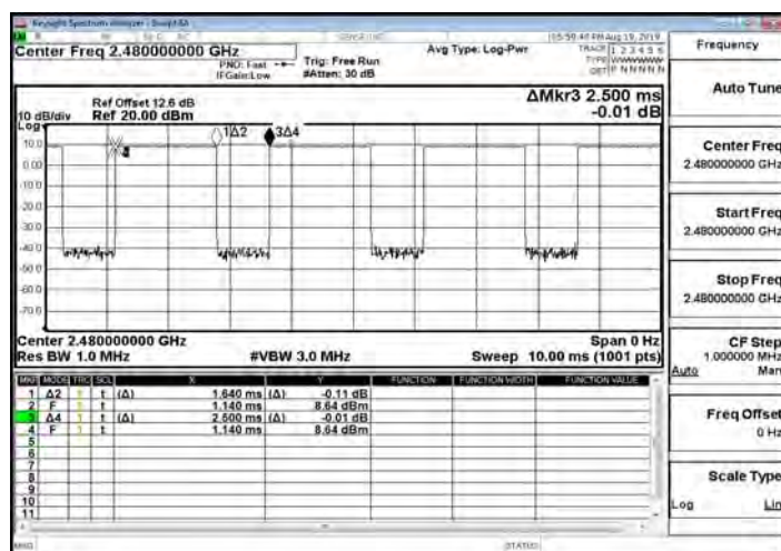
Dwell Time_GFSK_1M_DH3_2480MHz
