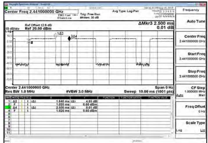
Dwell Time_π/4DQPSK_2M_DH5_2441MHz
