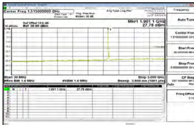
30MHz~3GHz_Band2_10MHz_QPSK_1_0_HighCH19150-1905
