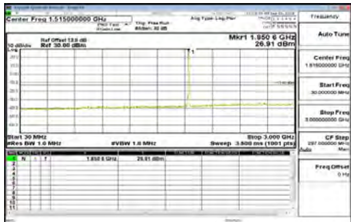
30MHz~3GHz_Band2_5MHz_QPSK_1_0_LowCH18625-1852.5
