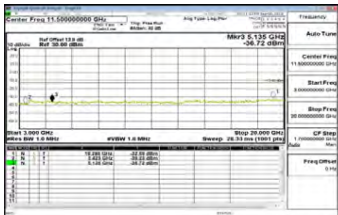
3GHz-20GHz_Band4_3MHz_QPSK_1_0_LowCH19965-1711.5
