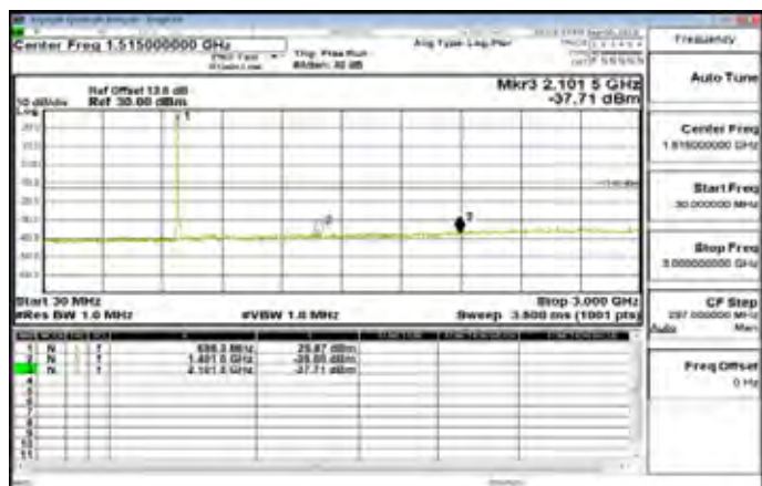
30MHz-3GHz_Band12_3MHz_QPSK_1_0_LowCH23025-700.5
