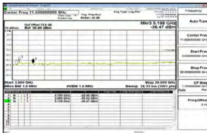
3GHz~20GHz_Band4_10MHz_QPSK_1_0_MidCH20175-1732.5
