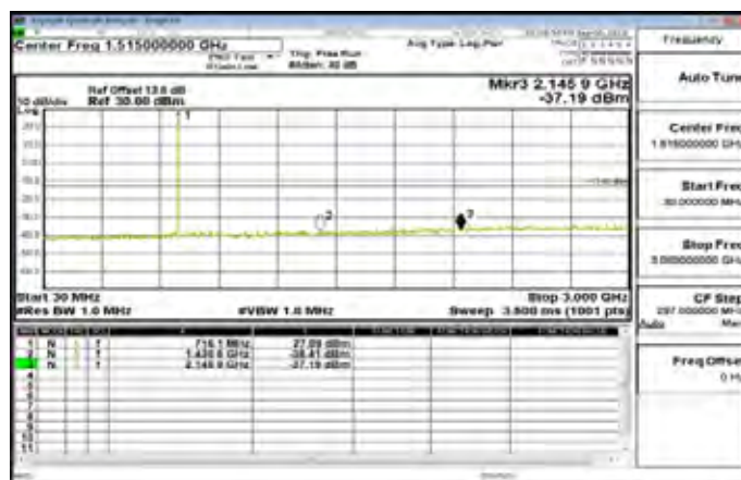
30MHz~3GHz_Band12_1_4MHz_QPSK_1_0_HighCH23173-715.3
