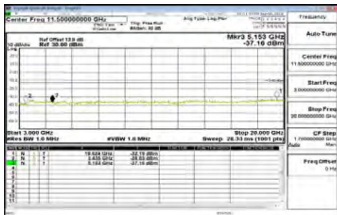
3GHz~20GHz_Band4_15MHz_QPSK_1_0_LowCH20025-1717.5
