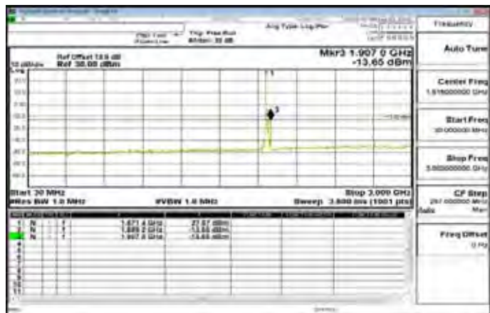
30MHz-3GHz_Band2_20MHz_QPSK_1_0_MidCH18900-1880
