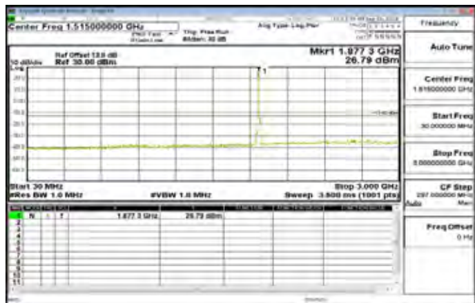
30MHz~3GHz_Band2_10MHz_QPSK_1_0_MidCH18900-1880
