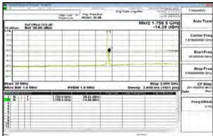
30MHz~3GHz_Band4_20MHz_QPSK_1_0_MidCH20175-1732.5
