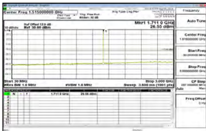
30MHz-3GHz_Band4_1_4MHz_QPSK_1_0_LowCH19957-1710.7
