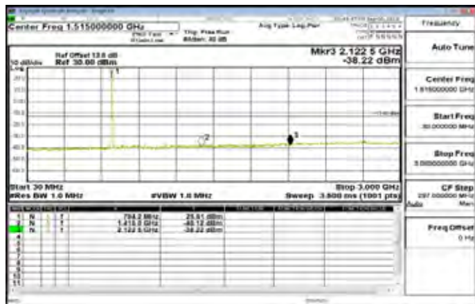
30MHz-3GHz_Band12_5MHz_QPSK_1_0_MidCH23095-707.5
