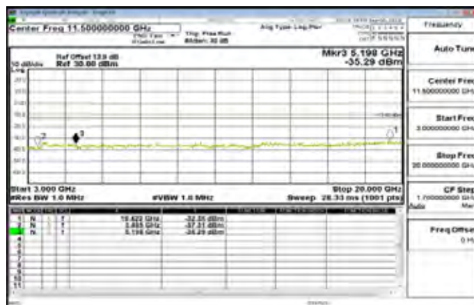
3GHz-20GHz_Band4_1_4MHz_QPSK_1_0_MidCH20175-1732.5
