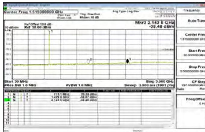
30MHz-3GHz_Band12_3MHz_QPSK_1_0_HighCH23165-714.5
