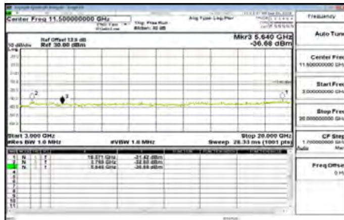
3GHz~20GHz_Band2_10MHz_QPSK_1_0_MidCH18900-1880
