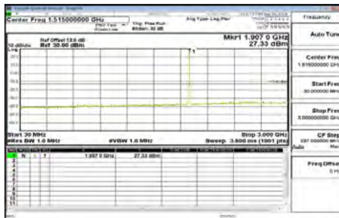
30MHz~3GHz_Band2_5MHz_QPSK_1_0_HighCH19175-1907.5
