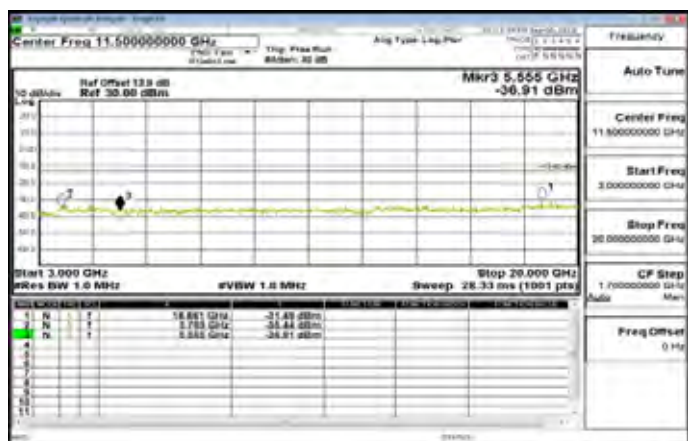
3GHz~20GHz_Band2_3MHz_QPSK_1_0_LowCH18615-1851.5
