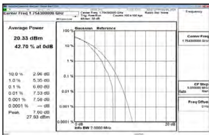
LTE_Band4_1_4MHz_16QAM_6_0_HighCH20393-1754.3
