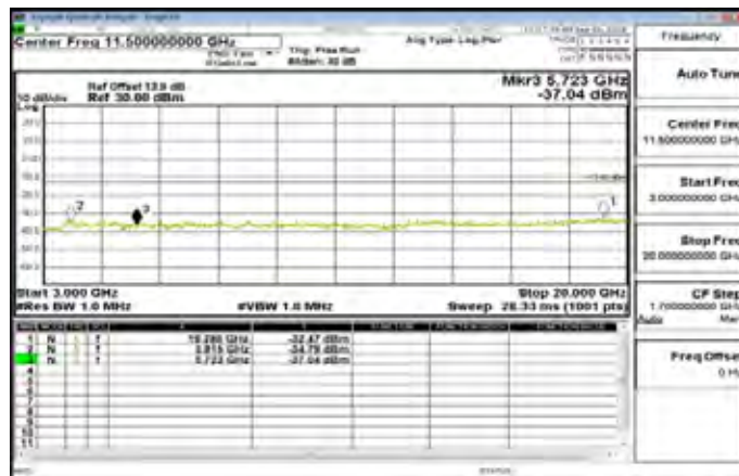
3GHz~20GHz_Band2_5MHz_QPSK_1_0_HighCH19175-1907.5
