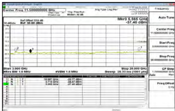
3GHz~20GHz_Band2_10MHz_QPSK_1_0_LowCH18650-1855
