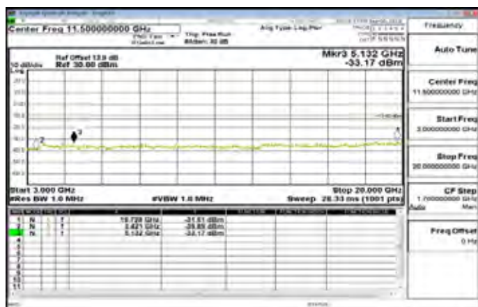
3GHz-20GHz_Band4_1_4MHz_QPSK_1_0_LowCH19957-1710.7
