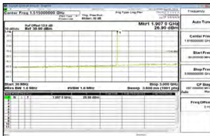
30MHz~3GHz_Band2_3MHz_QPSK_1_0_HighCH19185-1908.5
