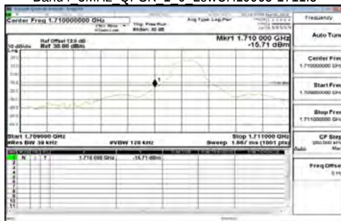
Band4 3MHz QPSK 1 0 LowCH19965-1711.5
