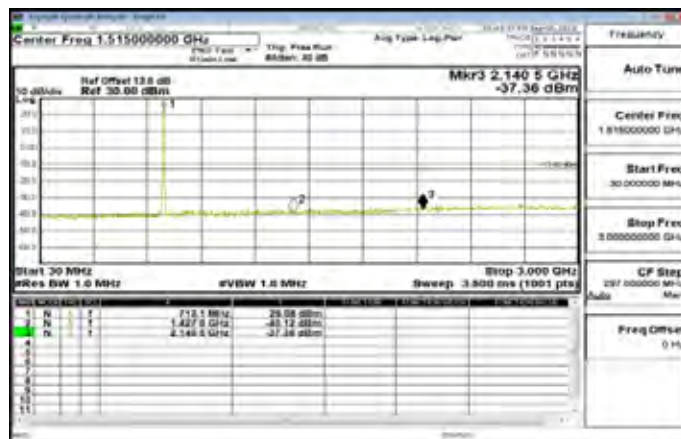
30MHz-3GHz_Band12_5MHz_QPSK_1_0_HighCH23155-713.5
