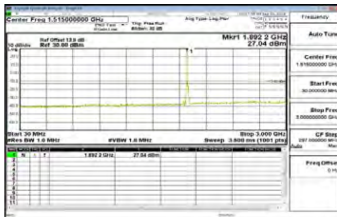
30MHz-3GHz_Band2_20MHz_QPSK_1_0_HighCH19100-1900
