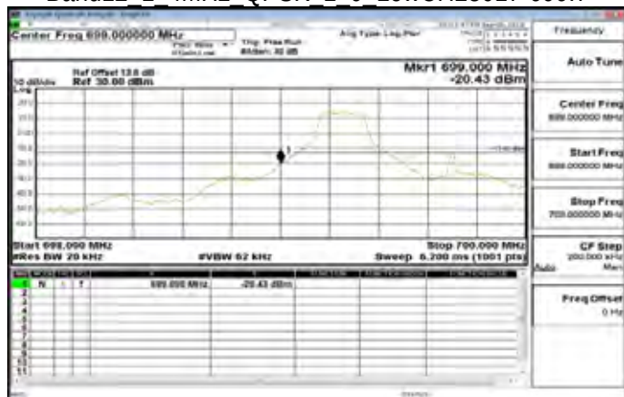
Band12 1 4MHz QPSK 1 0 LowCH23017-699.7
