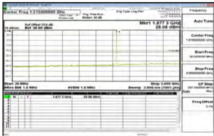
30MHz~3GHz_Band2_5MHz_QPSK_1_0_MidCH18900-1880
