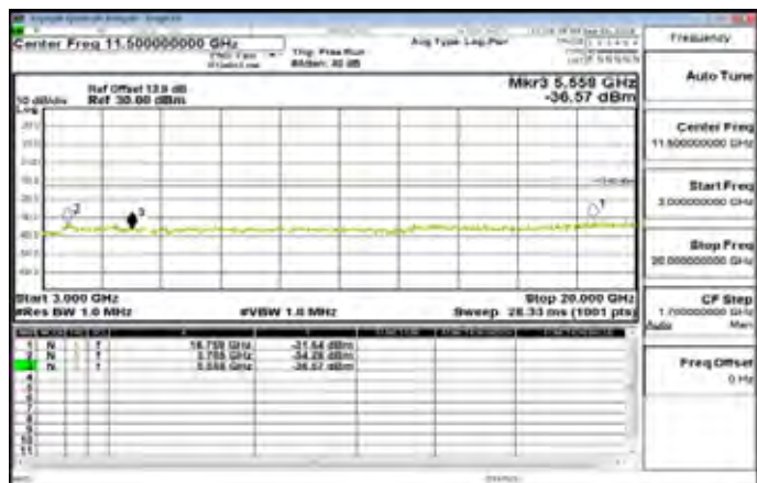
3GHz~20GHz_Band2_5MHz_QPSK_1_0_LowCH18625-1852.5
