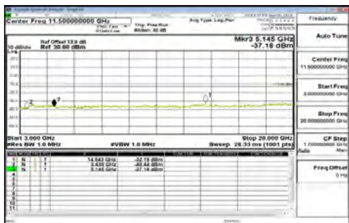
3GHz~20GHz_Band4_10MHz_QPSK_1_0_LowCH20000-1715
