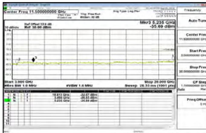
3GHz~20GHz_Band4_20MHz_QPSK_1_0_HighCH20300-1745
