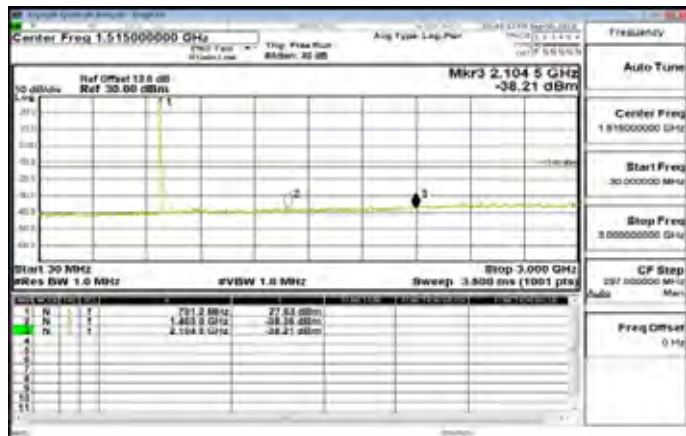
30MHz-3GHz_Band12_5MHz_QPSK_1_0_LowCH23035-701.5
