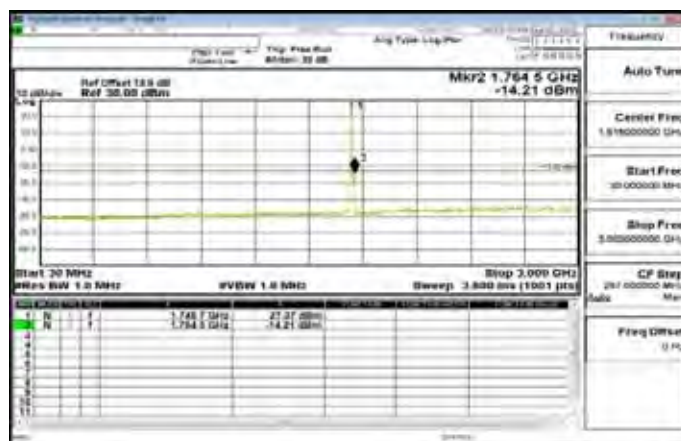
30MHz~3GHz_Band4_10MHz_QPSK_1_0_HighCH20350-1750
