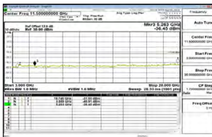
3GHz-20GHz_Band4_1_4MHz_QPSK_1_0_HighCH20393-1754.3
