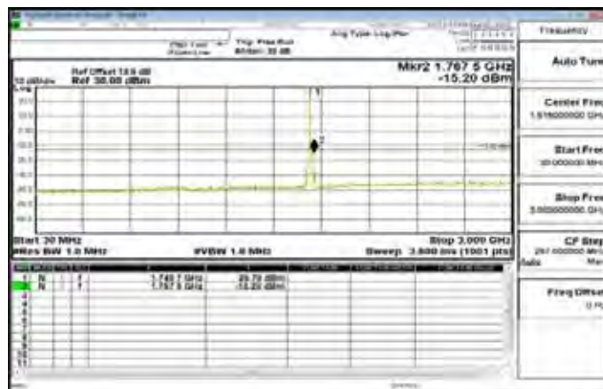
30MHz~3GHz_Band4_15MHz_QPSK_1_0_HighCH20325-1747.5
