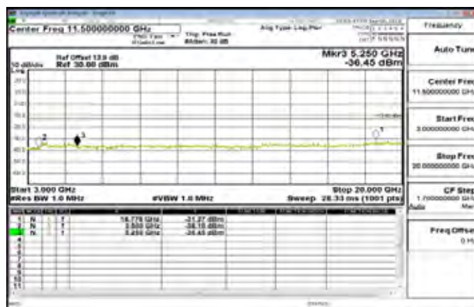
3GHz~20GHz_Band4_10MHz_QPSK_1_0_HighCH20350-1750
