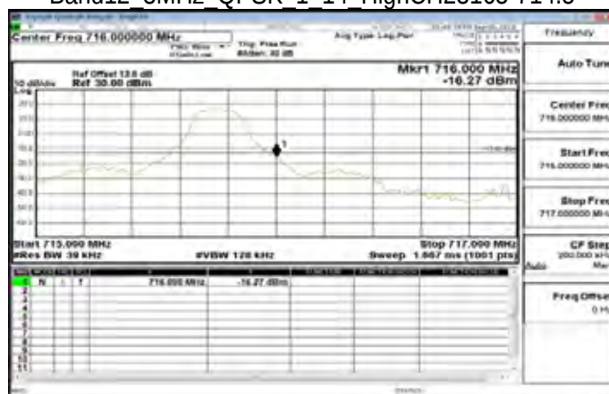
Band12 3MHz QPSK 1 14 HighCH23165-714.5
