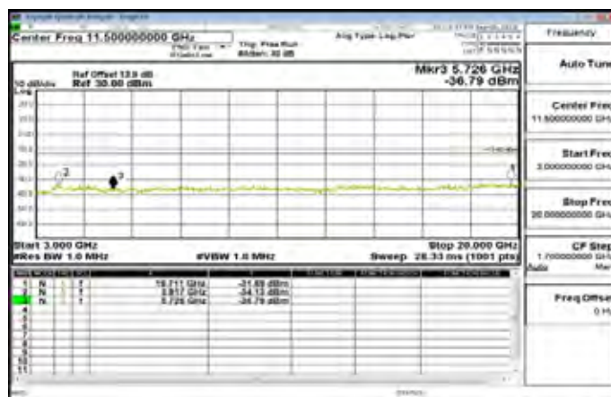
3GHz~20GHz_Band2_3MHz_QPSK_1_0_HighCH19185-1908.5
