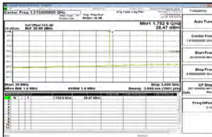
30MHz-3GHz_Band4_3MHz_QPSK_1_0_HighCH20385-1753.5
