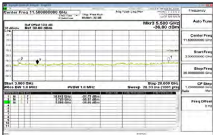
3GHz-20GHz_Band2_20MHz_QPSK_1_0_LowCH18700-1860
