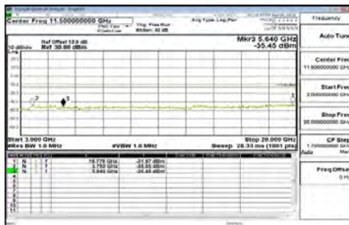
3GHz~20GHz_Band2_3MHz_QPSK_1_0_MidCH18900-1880
