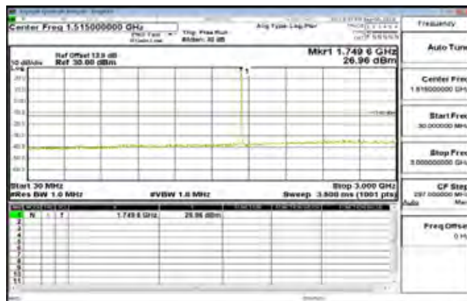
30MHz-3GHz_Band4_5MHz_QPSK_1_0_HighCH20375-1752.5
