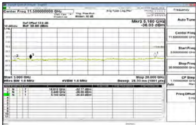
3GHz~20GHz_Band4_20MHz_QPSK_1_0_LowCH20050-1720
