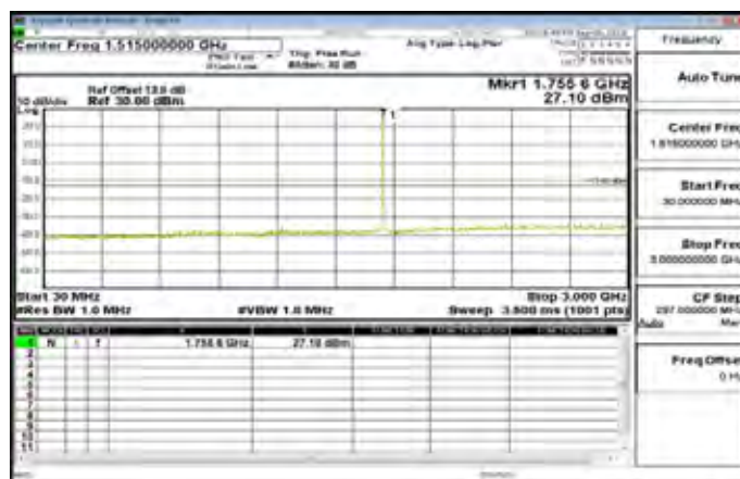
30MHz-3GHz_Band4_1_4MHz_QPSK_1_0_HighCH20393-1754.3
