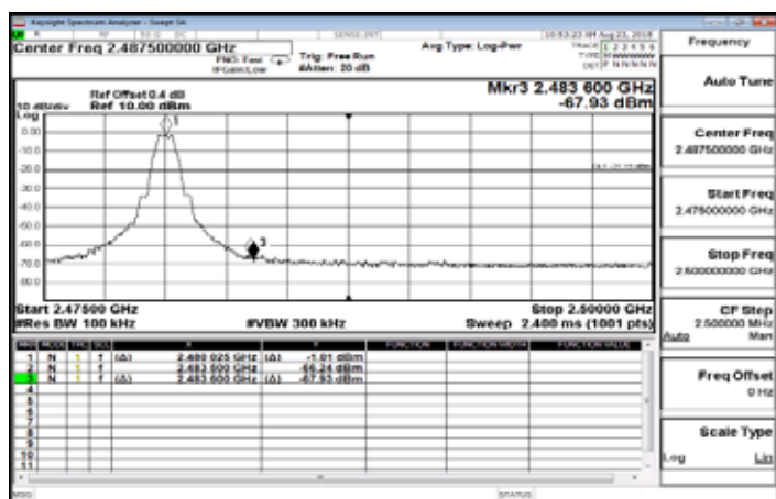
Band Edge_BLE_1M_HighCH39-2480
