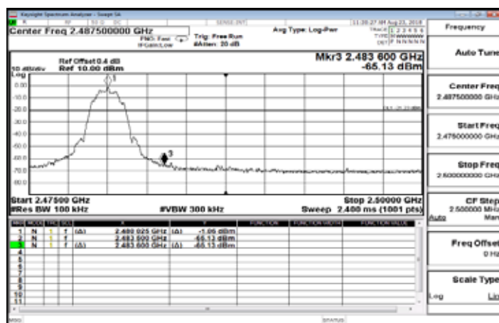
Band Edge_BLE_2M_HighCH39-2480
