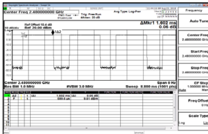
Dwell Time_GFSK_1M_DH3_2480MHz
