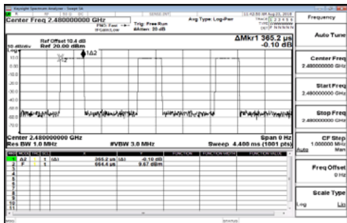
Dwell Time_GFSK_1M_DH1_2480MHz
