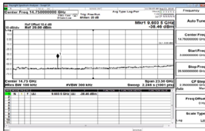
Spurious Emission High_GFSK_1M_DH5_2441MHz
