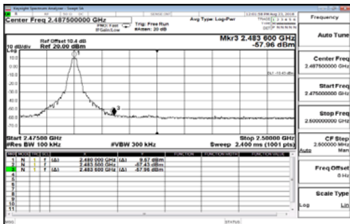
Band Edge_GFSK_1M_DH5_2480MHz
