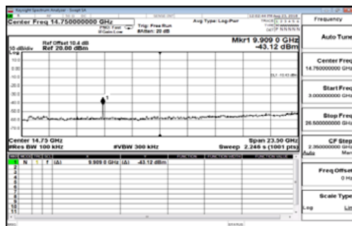
Spurious Emission High_GFSK_1M_DH5_2480MHz
