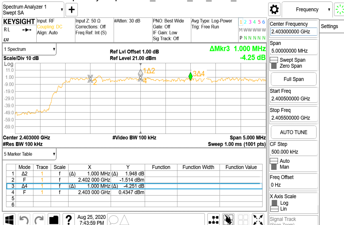
Frequency Separation_8DPSK_3M_DH5_CH0CH1CH2
