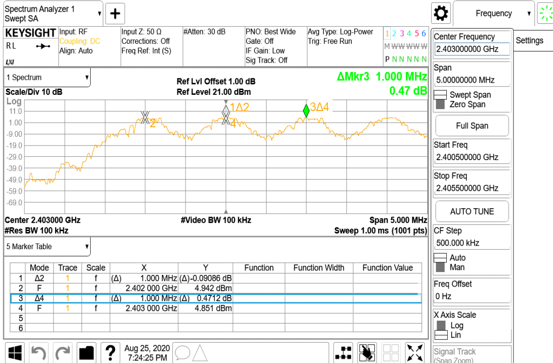
Frequency Separation_8DPSK_3M_DH5_CH0CH1CH2
