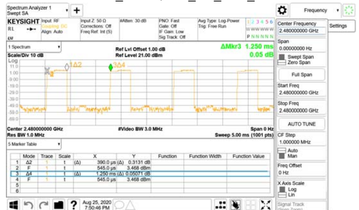
Dwell Time_π/4DQPSK_2M_DH1_2480MHz
