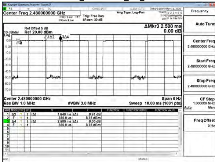
Dwell Time_π/4DQPSK_2M_2480MHz
