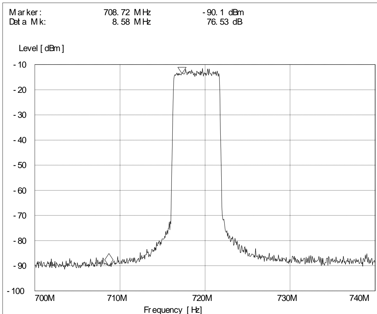
Figure 6-13: Power of the MediaFlo transmitter
