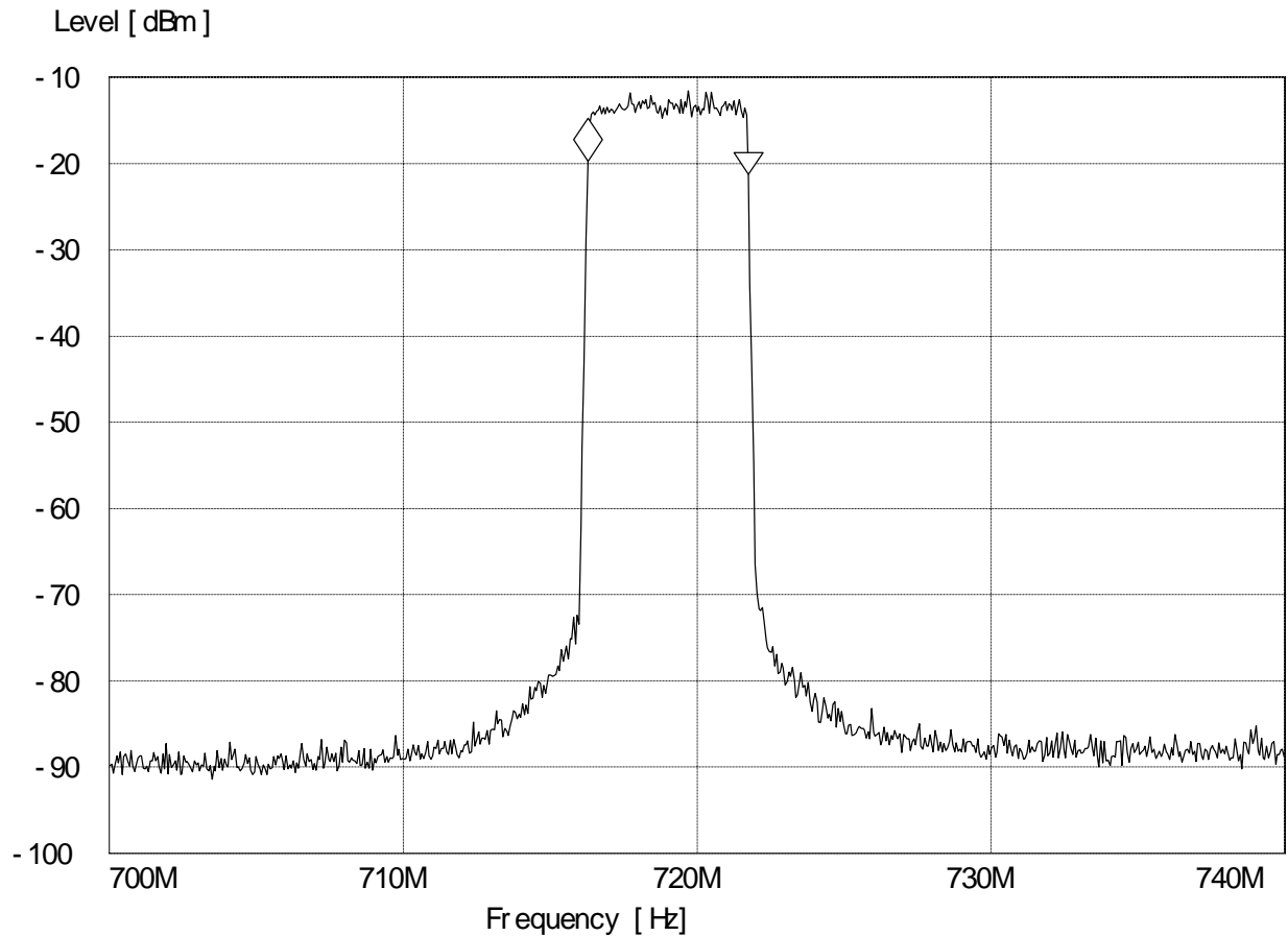
Figure 6-12 Bandwidth of the MediaFlo transmitter
