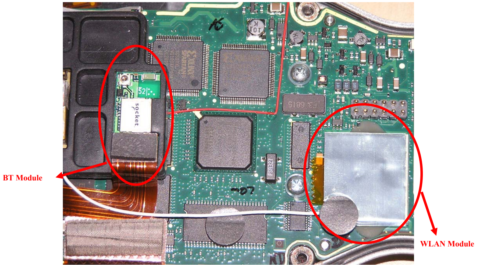
EUT – Open view identifying BT and WLAN modules
