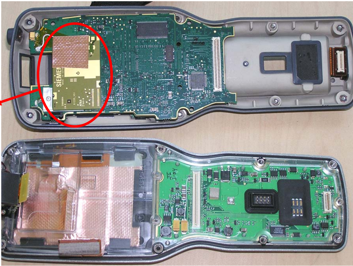
EUT Open view – showing GSM module
