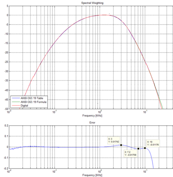
Figure 39.3: Spectral filter for convolution and deviation from the target defined in the standard [1]. Worst case deviation is < 0.02 dB in the frequency range from 10 Hz to 10 kHz.
