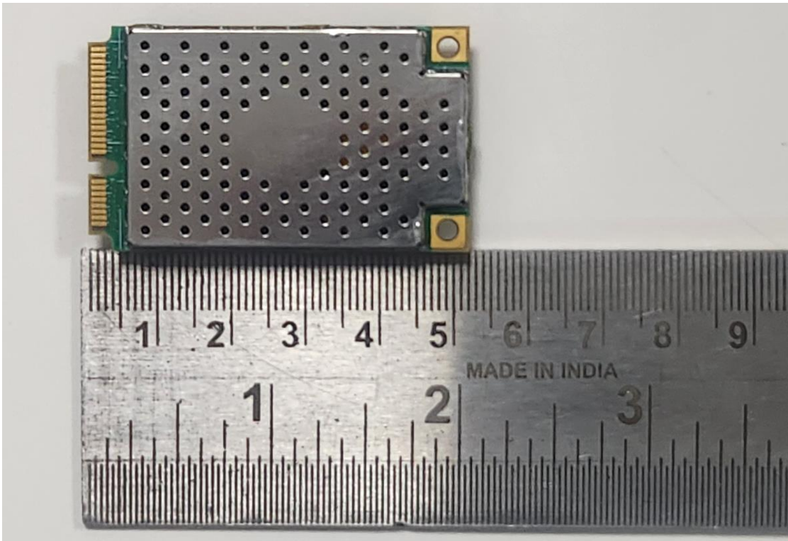
IM21-PRT RFID Module dimension (Length = 50.85mm)
