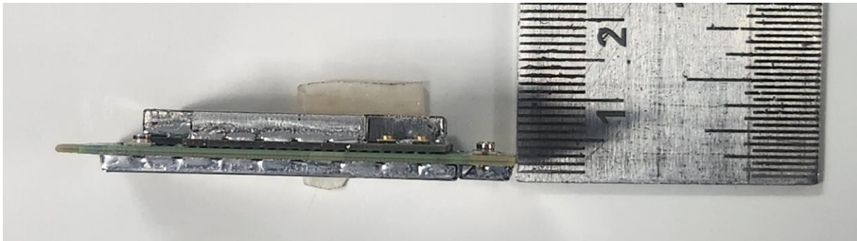
IM21-PRT RFID Module dimension (Height = 7.18mm)
