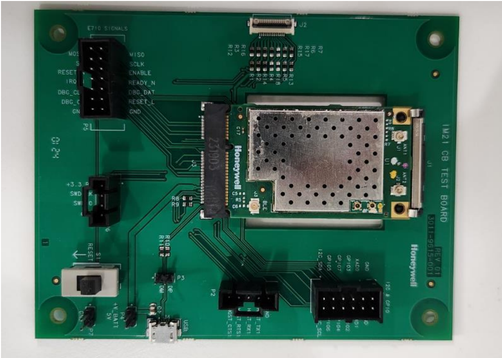
IM21-PRT RFID Module inserted in test board (only for testing purpose) – Top View
