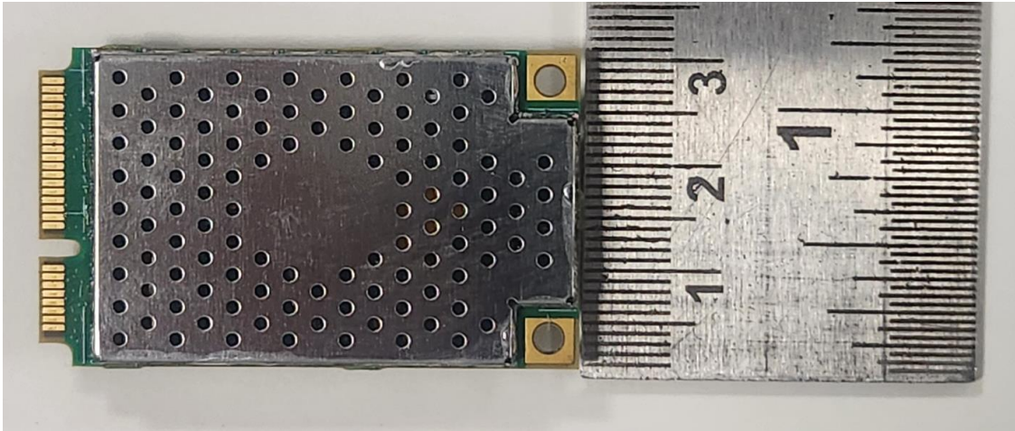
IM21-PRT RFID Module dimension (Width = 30.43mm)
