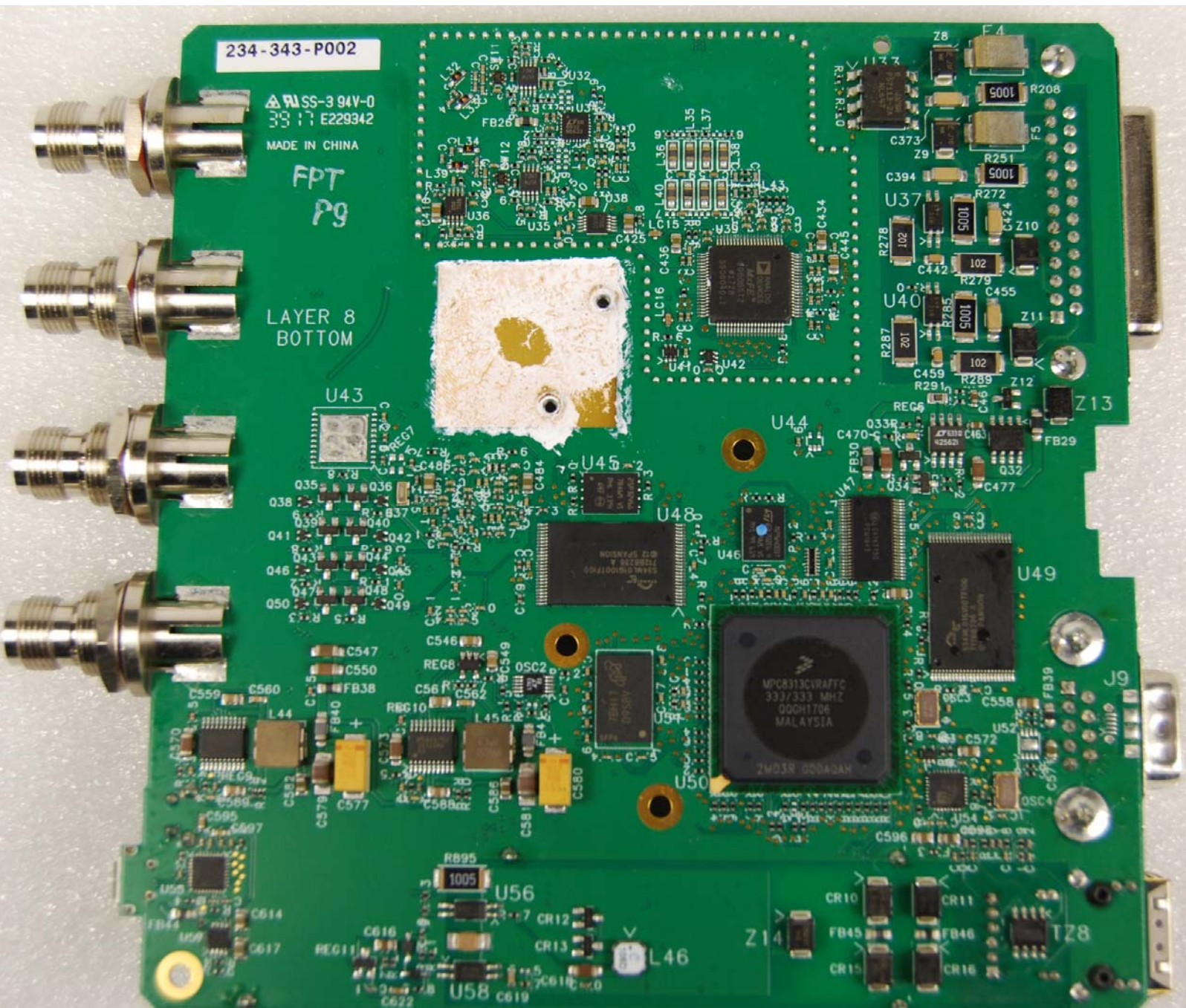
Bottom Side (Shield Removed)
