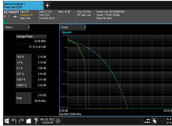
N14(5M)_DFT-s-OFDM_PI_2-BPSK_Edge_1RB_Left_High_CH
