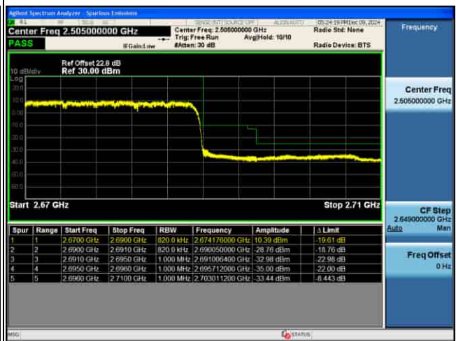
EDGE_5G_n41_30KHz_Pi2-BPSK_50M_1RB@MAX_CH532998
