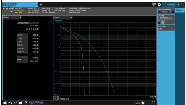
PAPR_5G_n66_15KHz_40M_1745MHz-64QAM
