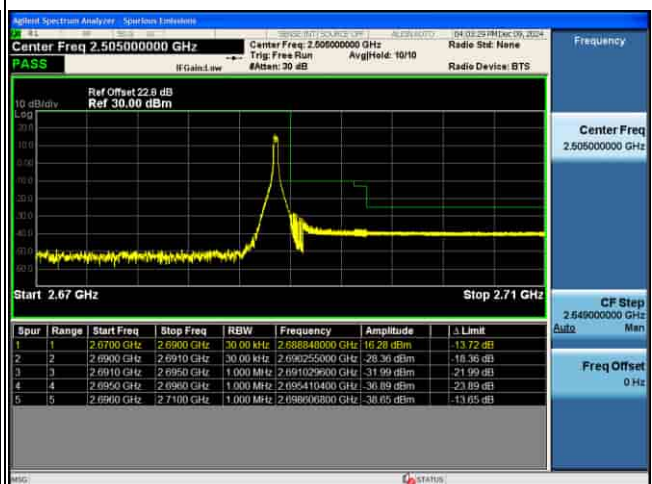
EDGE_5G_n41_30KHz_Pi2-BPSK_80M_FULL RB@MAX_CH529998
