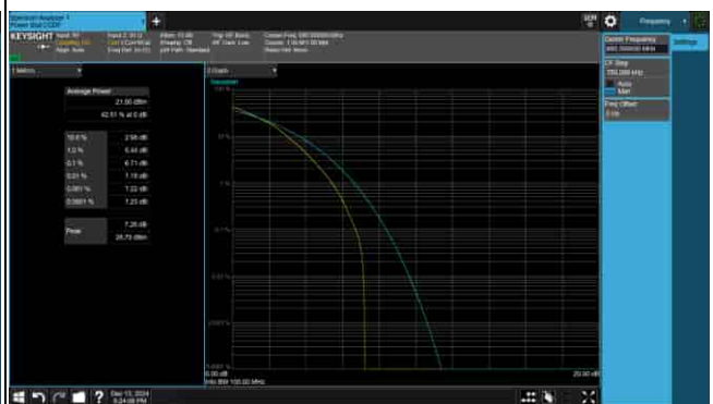
PAPR_5G_n71_15KHz_10M_680.5MHz-64QAM
