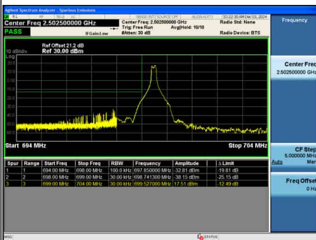
EDGE_5G_n12_15KHz_Pi2-BPSK_15M_FULL RB@0_CH141300
