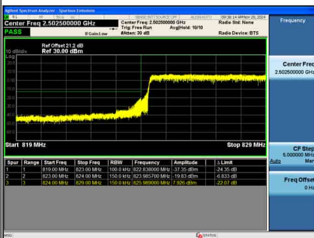
EDGE_5G_n26_15KHz_Pi2-BPSK_15M_FULL RB@0_CH166300
