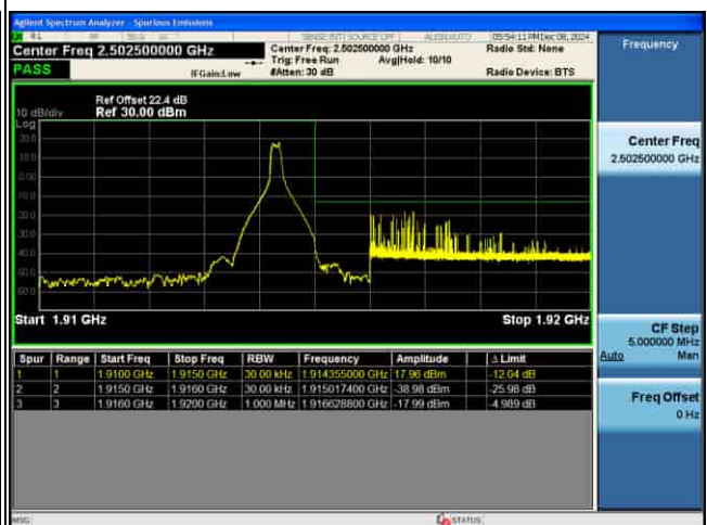
EDGE_5G_n25_15KHz_Pi2-BPSK_30M_FULL RB@MAX_CH380000
