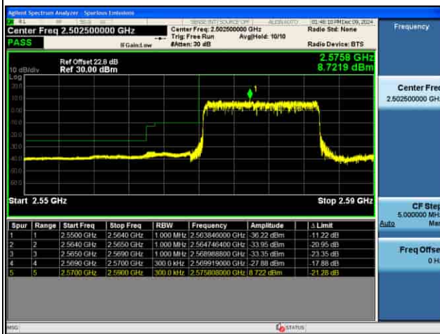
EDGE_5G_n38_30KHz_Pi2-BPSK_20M_1RB@0_CH516000
