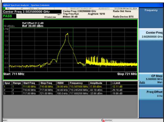
EDGE_5G_n12_15KHz_Pi2-BPSK_15M_FULL RB@MAX_CH141700
