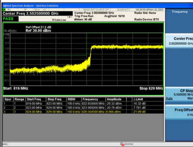
EDGE_5G_n26_15KHz_Pi2-BPSK_15M_1RB@0_CH166300
