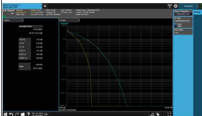
PAPR_5G_n66_15KHz_10M_1745MHz-16QAM
