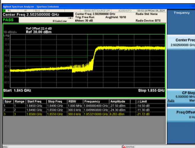
EDGE_5G_n25_15KHz_Pi2-BPSK_30M_FULL RB@0_CH373000
