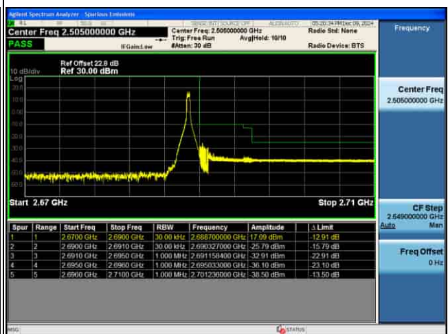
EDGE_5G_n41_30KHz_Pi2-BPSK_50M_FULL RB@MAX_CH532998
