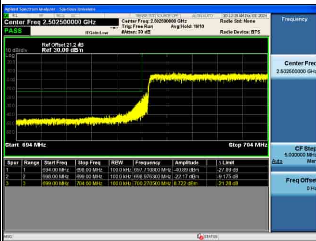
EDGE_5G_n12_15KHz_Pi2-BPSK_15M_1RB@0_CH141300
