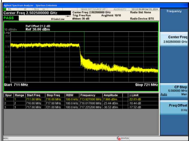
EDGE_5G_n12_15KHz_Pi2-BPSK_15M_1RB@MAX_CH141700
