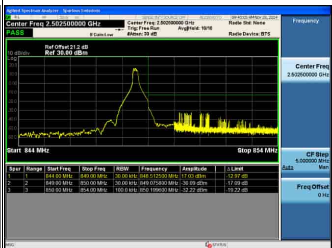
EDGE_5G_n26_15KHz_Pi2-BPSK_15M_FULL RB@MAX_CH168300
