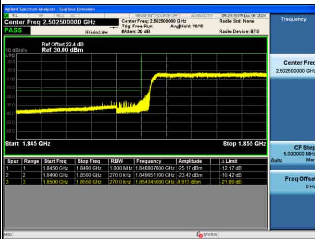
EDGE_5G_n25_15KHz_Pi2-BPSK_30M_1RB@0_CH373000
