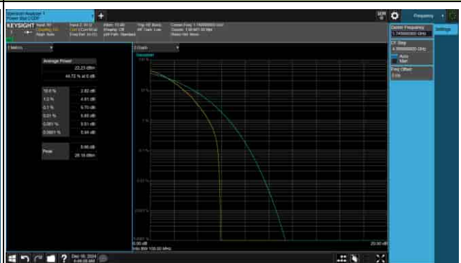
PAPR_5G_n66_15KHz_15M_1745MHz-64QAM
