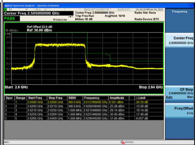
EDGE_5G_n38_30KHz_Pi2-BPSK_20M_1RB@MAX_CH522000
