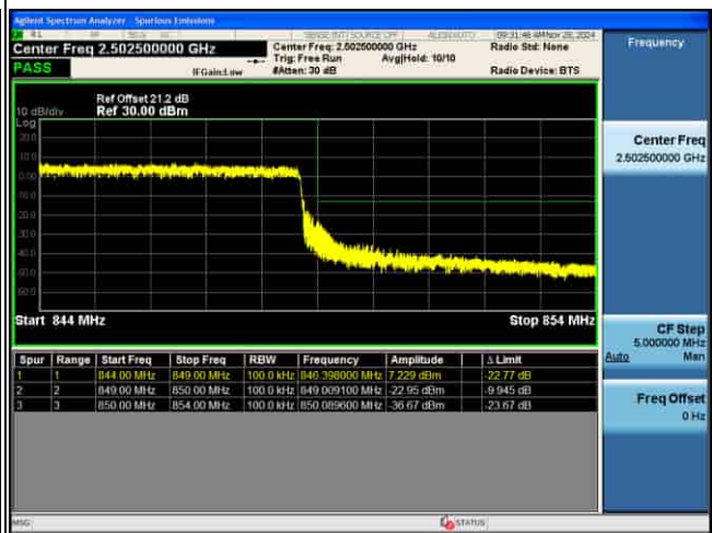
EDGE_5G_n26_15KHz_Pi2-BPSK_15M_1RB@MAX_CH168300
