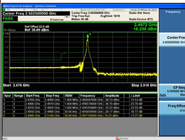
EDGE_5G_n41_30KHz_Pi2-BPSK_80M_FULL RB@0_CH507204
