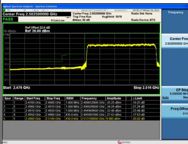
EDGE_5G_n41_30KHz_Pi2-BPSK_20M_FULL RB@0_CH501204
