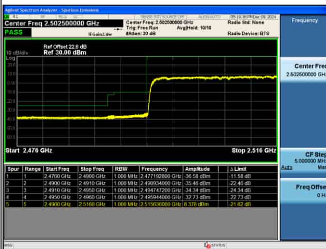
EDGE_5G_n41_30KHz_Pi2-BPSK_50M_FULL RB@0_CH504204
