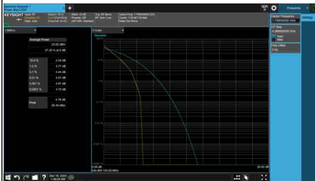
PAPR_5G_n66_15KHz_40M_1745MHz-16QAM
