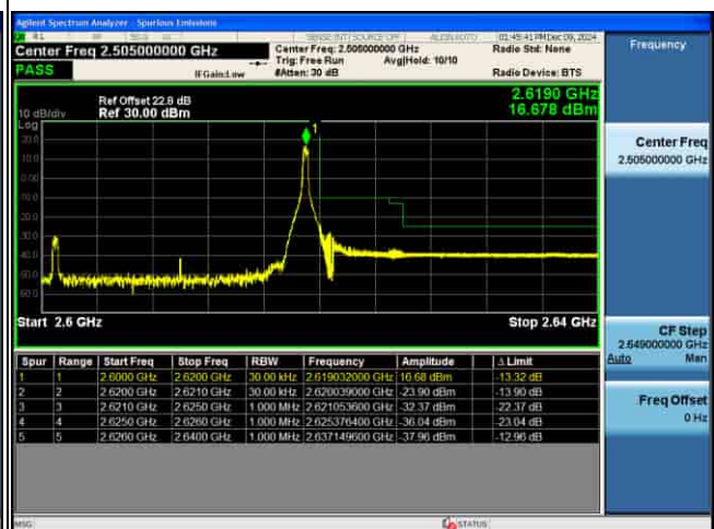
EDGE_5G_n38_30KHz_Pi2-BPSK_20M_FULL RB@MAX_CH522000
