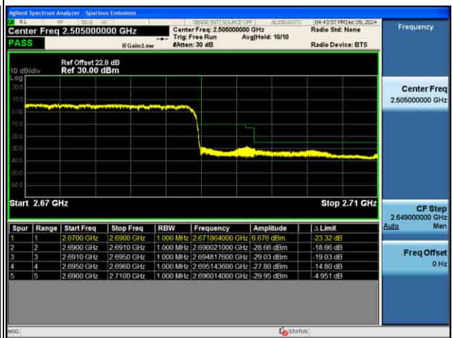
EDGE_5G_n41_30KHz_Pi2-BPSK_80M_1RB@MAX_CH529998
