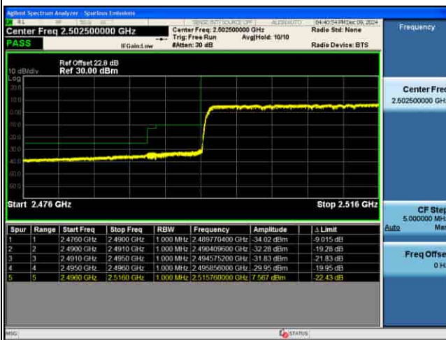
EDGE_5G_n41_30KHz_Pi2-BPSK_80M_1RB@0_CH507204
