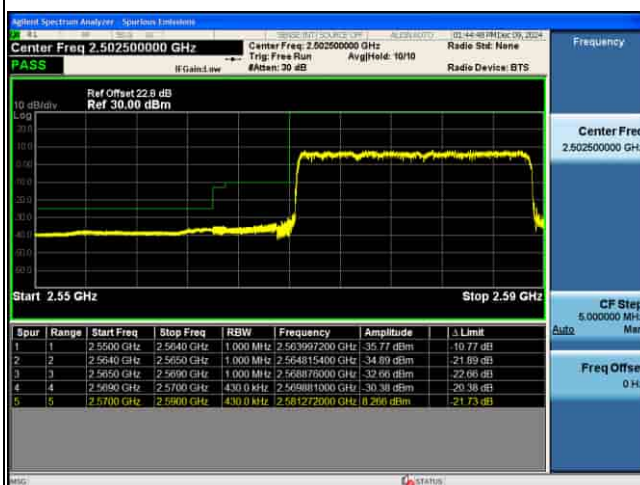
EDGE_5G_n38_30KHz_Pi2-BPSK_20M_FULL RB@0_CH516000
