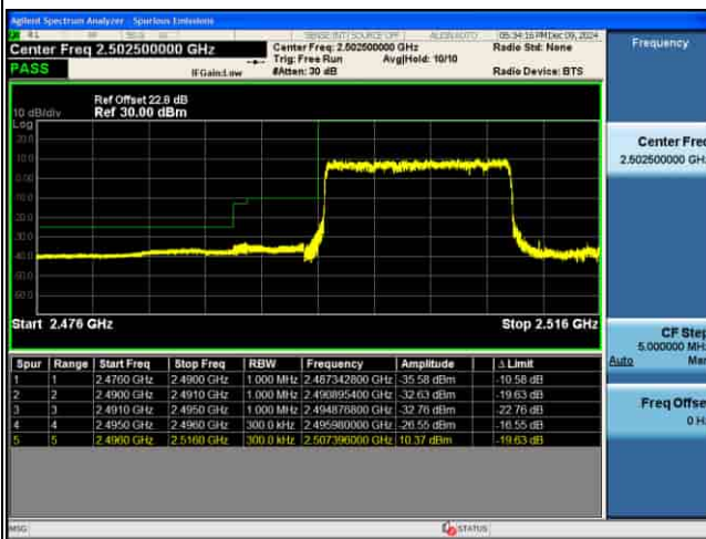
EDGE_5G_n41_30KHz_Pi2-BPSK_20M_1RB@0_CH501204
