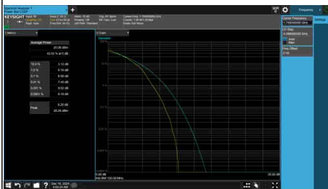
PAPR_5G_n66_15KHz_25M_1745MHz-256QAM
