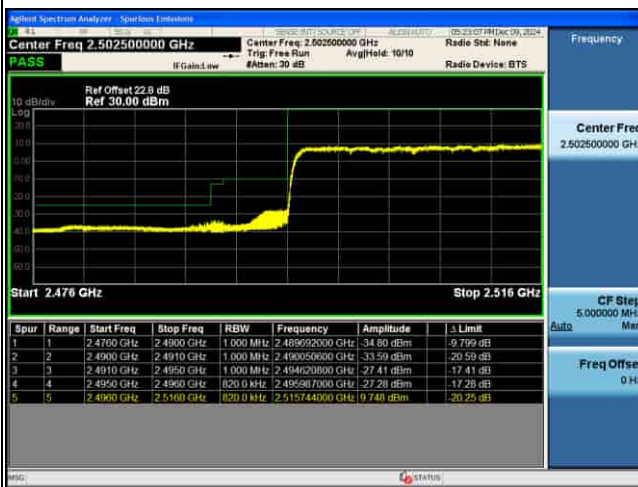
EDGE_5G_n41_30KHz_Pi2-BPSK_50M_1RB@0_CH504204
