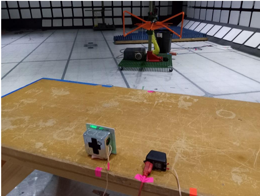
< 1 GHz setup
