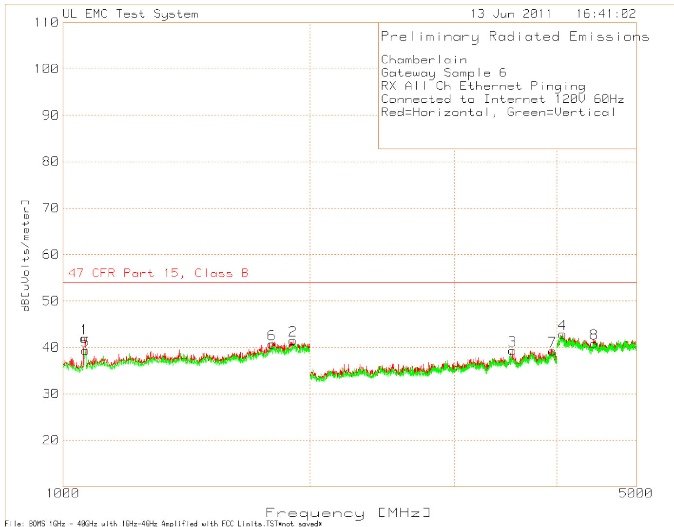
Figure 6 Radiated Emissions Graph 1GHz – 5GHz
