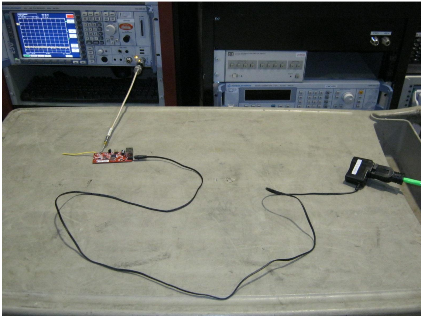
Figure 35 Test setup for Maximum Peak Output Power
