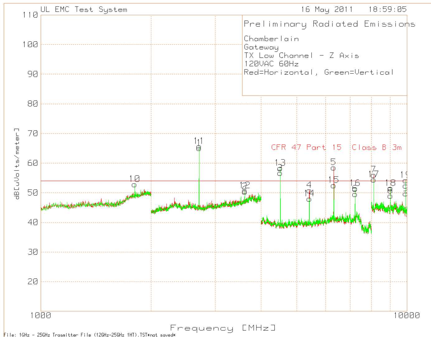
Figure 18 Radiated Spurious Emissions above 1GHz, Low Channel Z-axis
