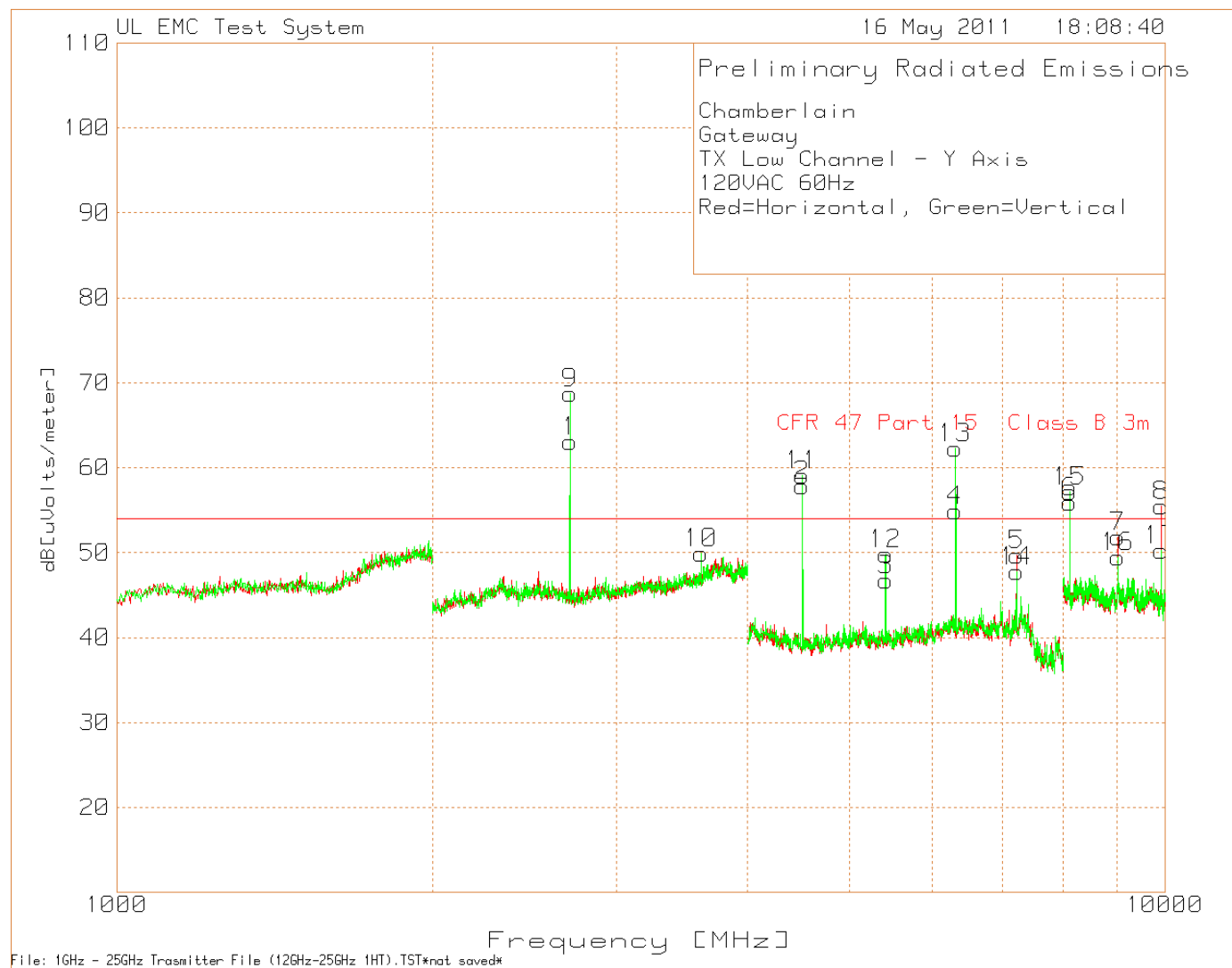
Figure 17 Radiated Spurious Emissions above 1GHz, Low Channel Y-axis
