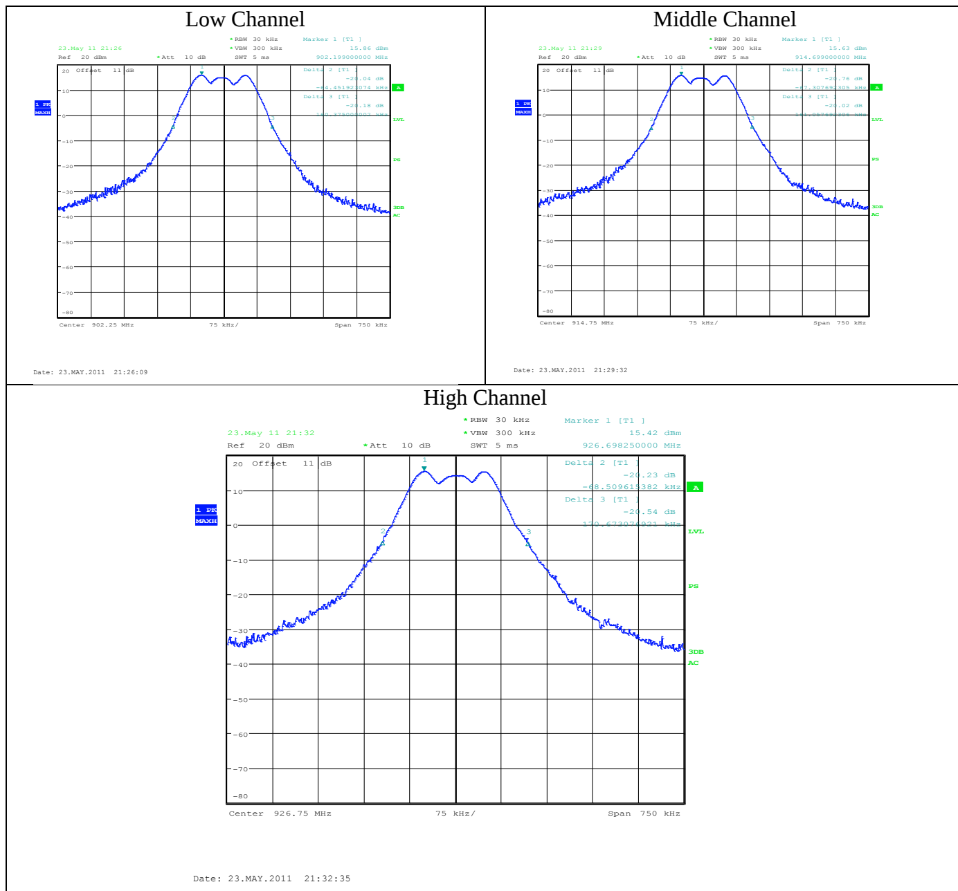
Figure 34 20dB Bandwidth Graphs
