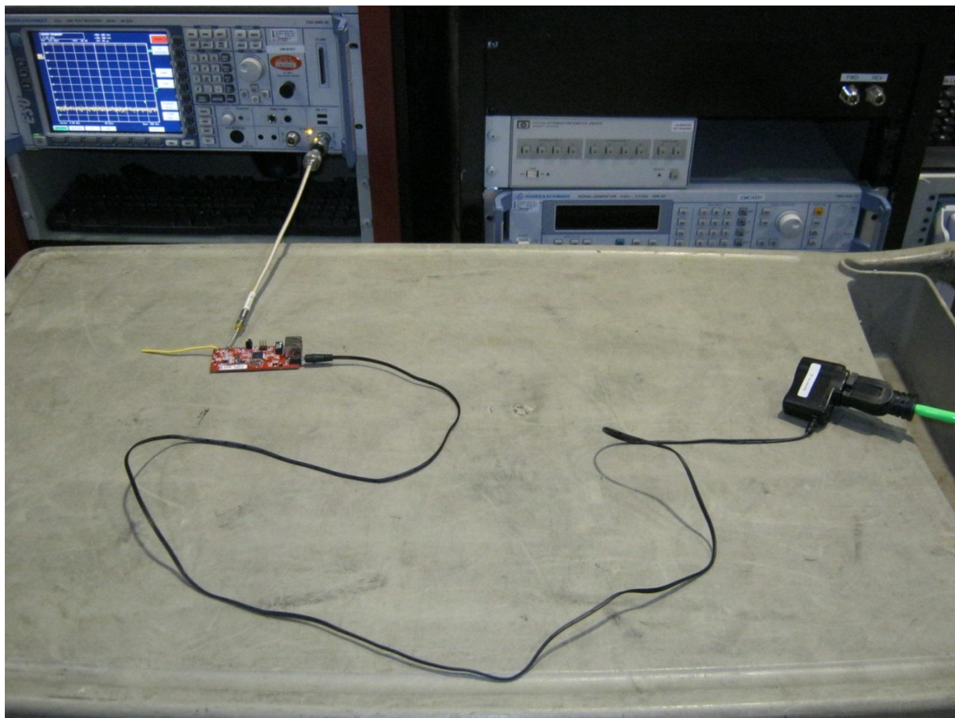
Figure 32 Test Setup for Dwell Time
