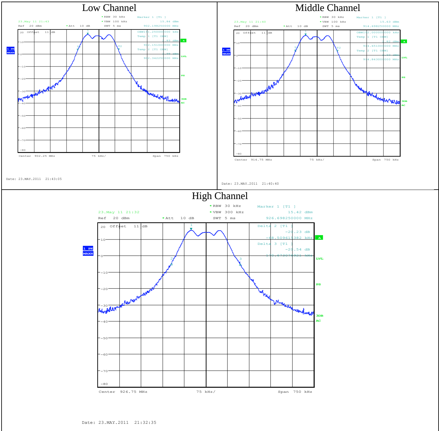
Figure 37 99% Power Bandwidth Graphs
