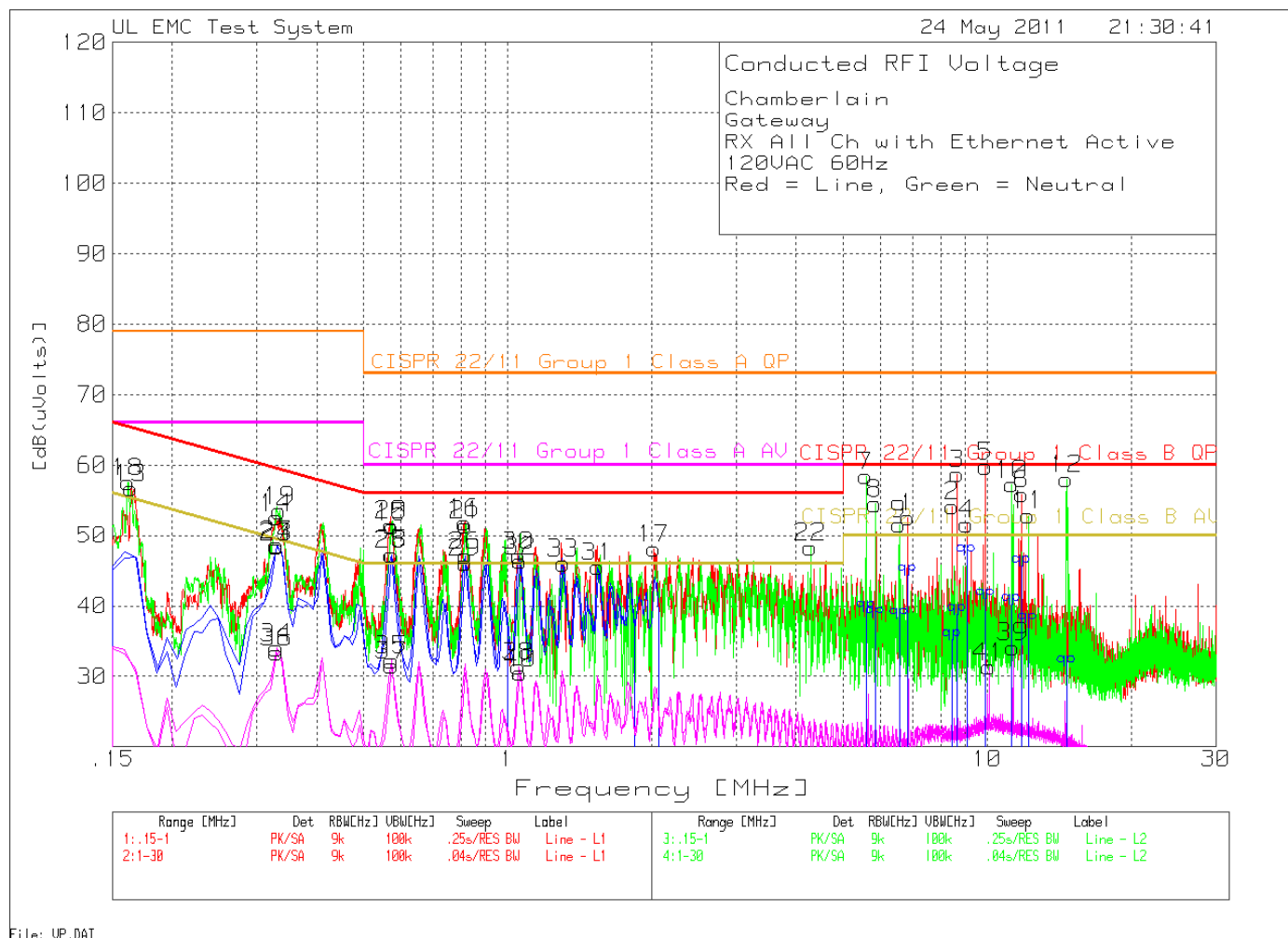
Figure 3 Conducted Emissions Graph – RX All Channels with Ethernet Active
