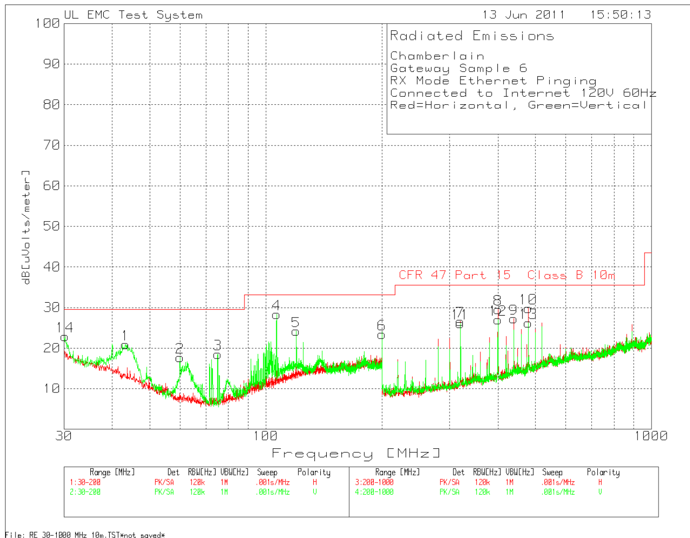
Figure 5 Radiated Emissions Graph 30MHz – 1GHz
