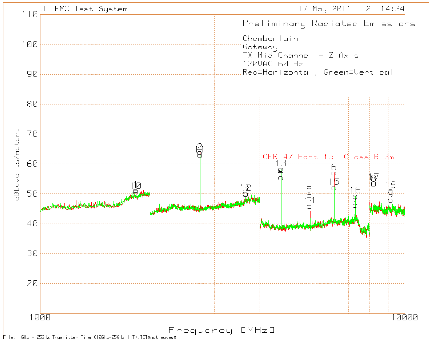
Figure 21 Radiated Spurious Emissions above 1GHz, Mid Channel Z-axis
