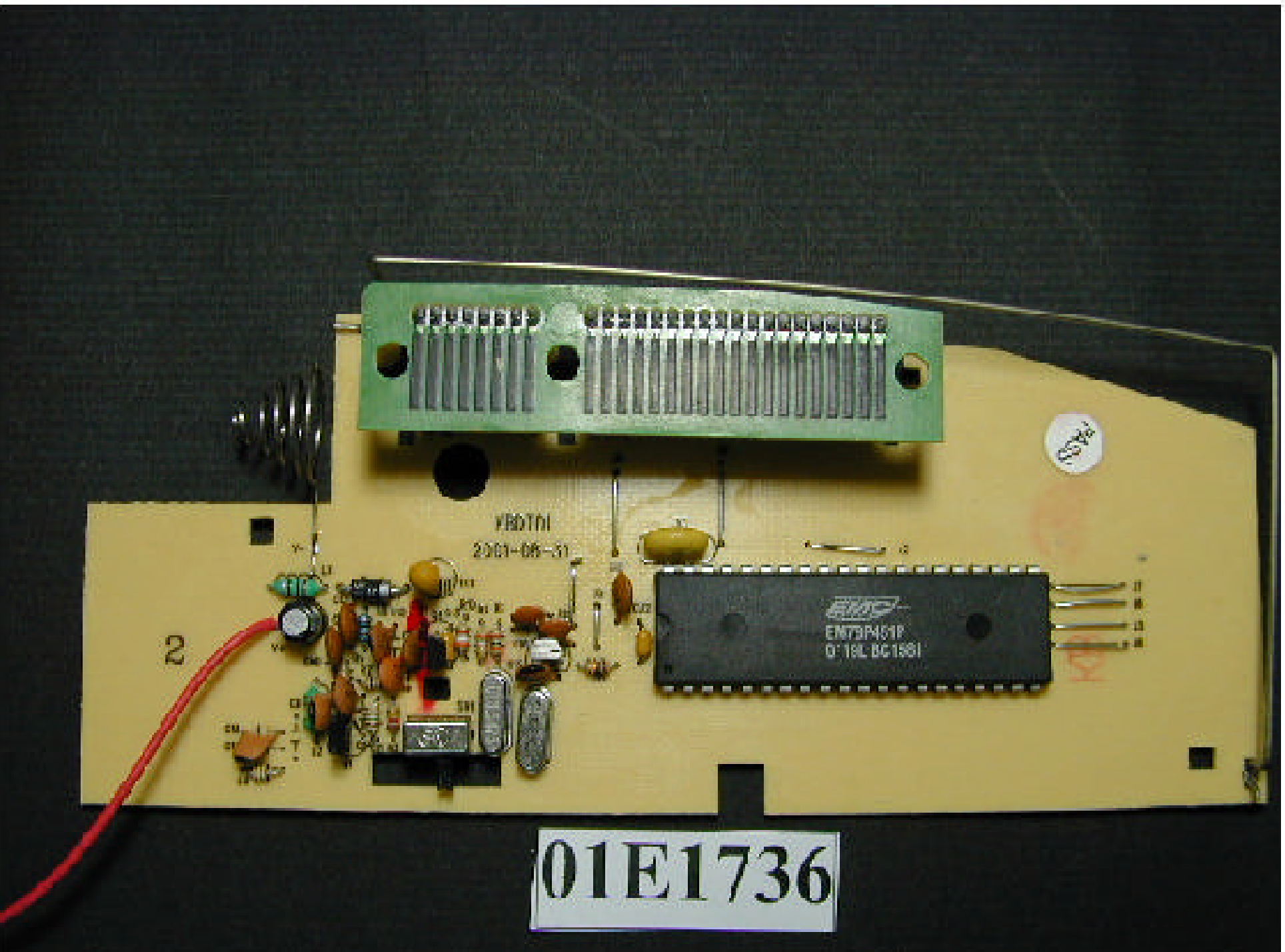
Photo # 5. Unit Partially Disassembled
