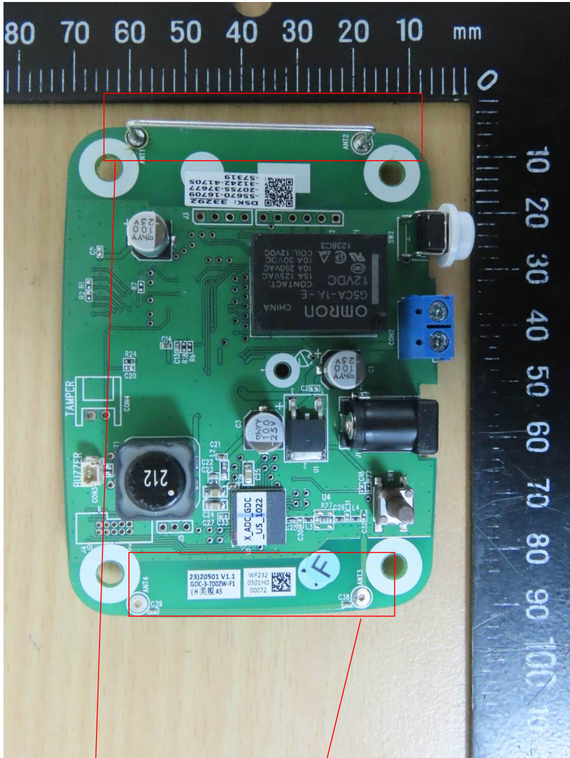
433MHz antenna
