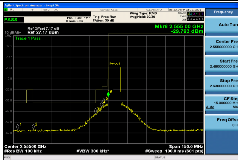
Band41-10MHz-16QAM-40290-50RB#0
