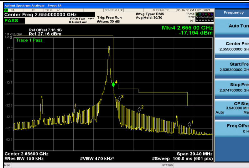
Band41-15MHz-16QAM-41165-1RB#74
