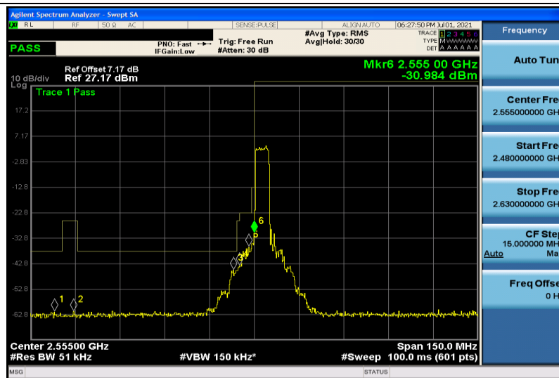
Band41-5MHz-QPSK-40265-25RB#0
