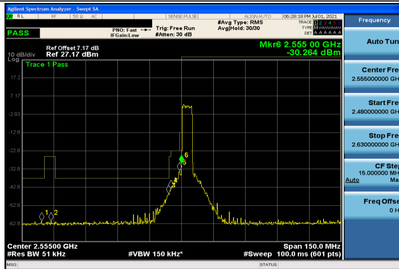
Band41-5MHz-16QAM-40265-25RB#0
