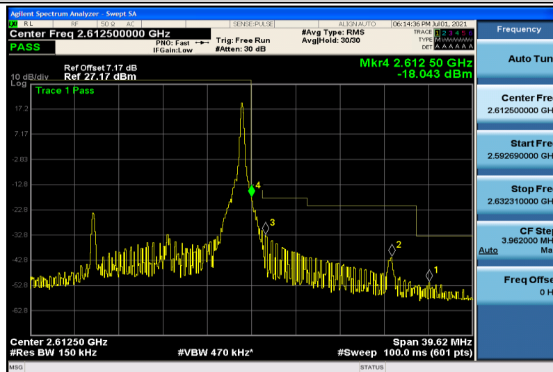
Band41-15MHz-16QAM-40740-1RB#74
