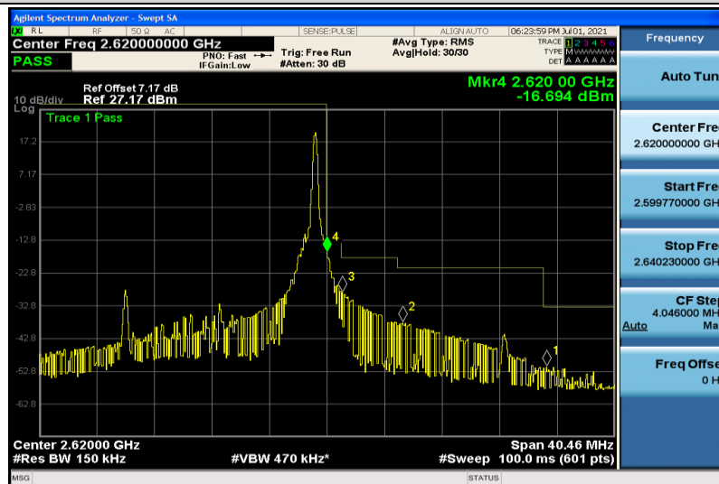
Band38-15MHz-16QAM-38175-1RB#74
