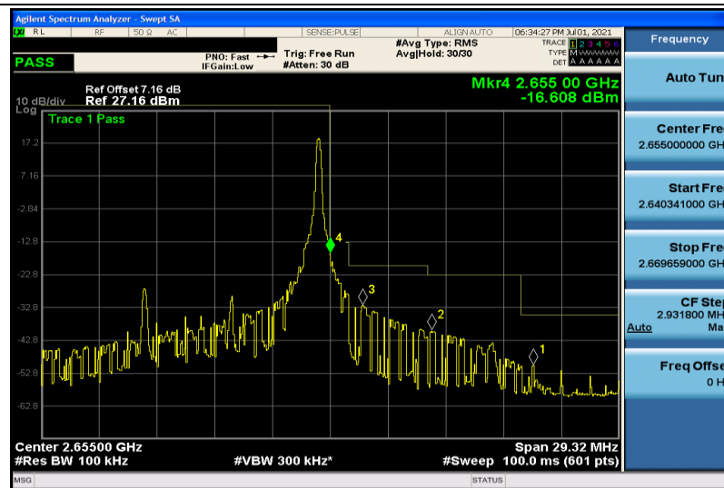
Band41-10MHz-16QAM-41190-1RB#49
