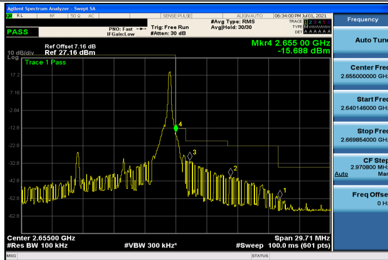
Band41-10MHz-QPSK-41190-1RB#49
