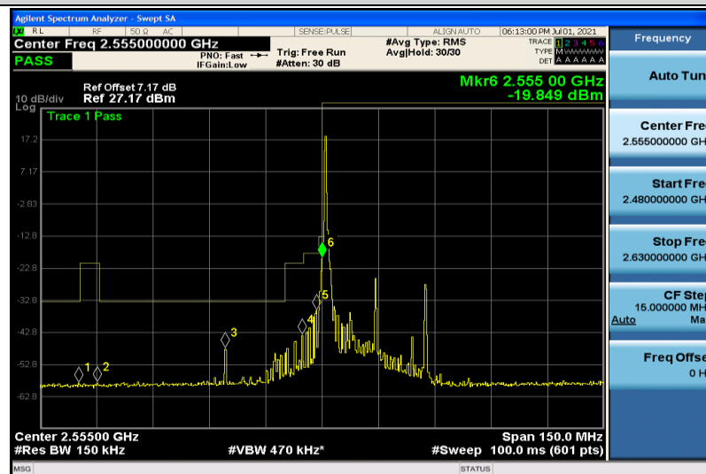
Band41-15MHz-QPSK-40315-1RB#0
