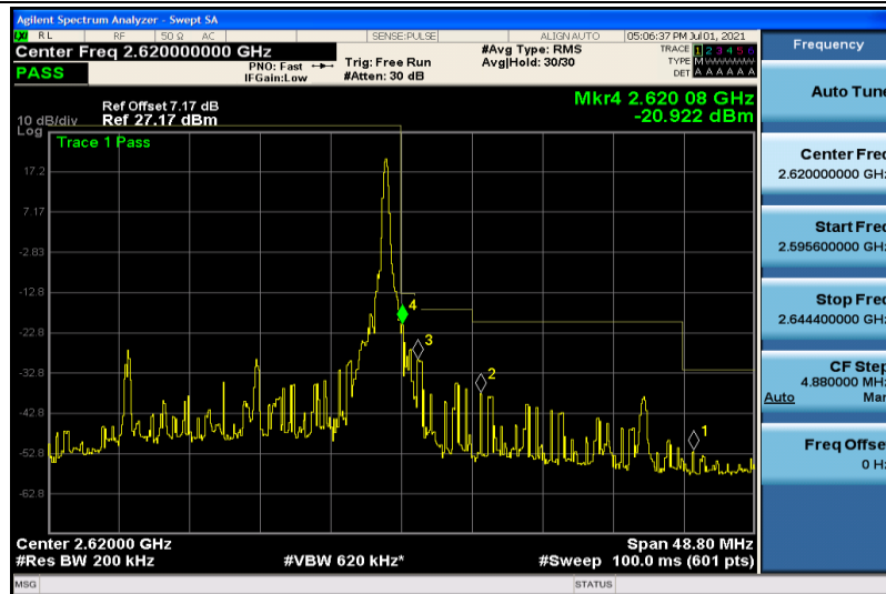
Band38-20MHz-16QAM-38150-1RB#99
