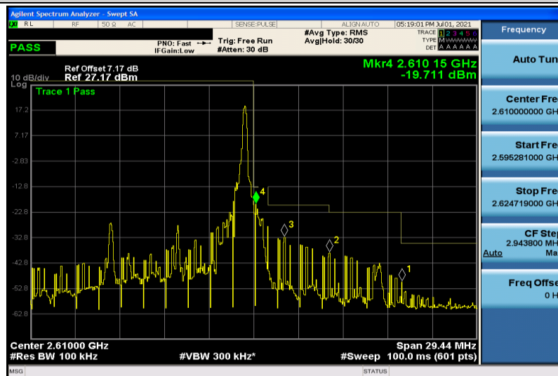
Band41-10MHz-16QAM-40740-1RB#49
