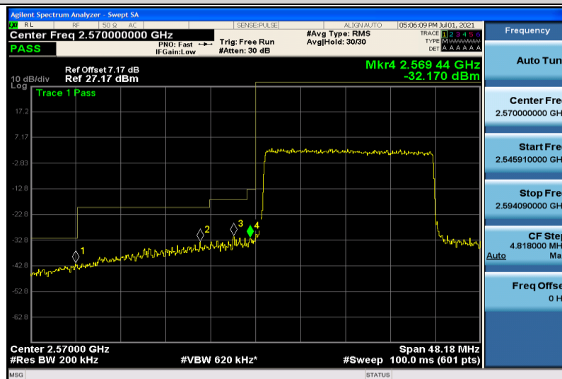
Band38-20MHz-16QAM-37850-100RB#0
