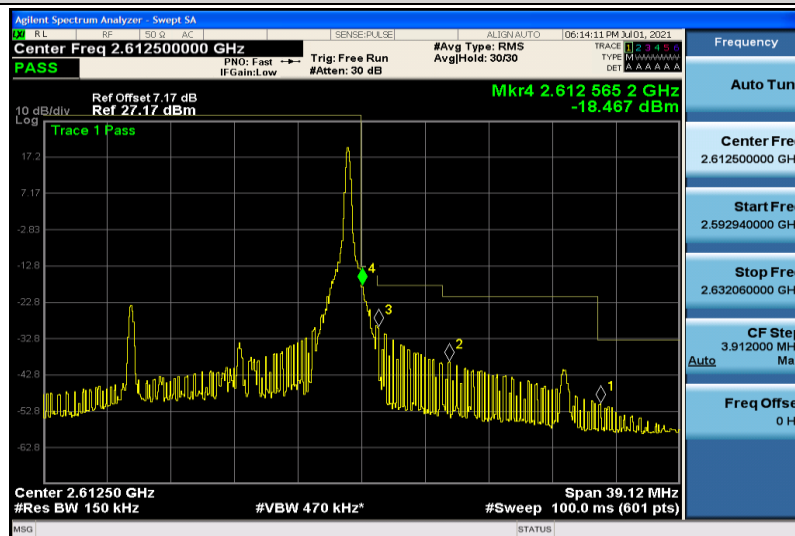
Band41-15MHz-QPSK-40740-1RB#74
