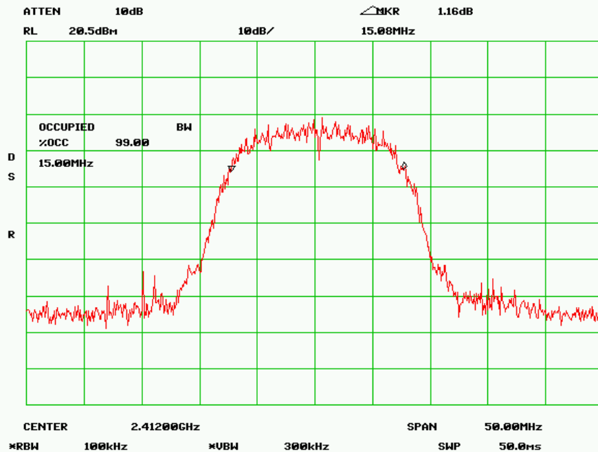
99% Bandwidth - Low Channel (802.11b)
