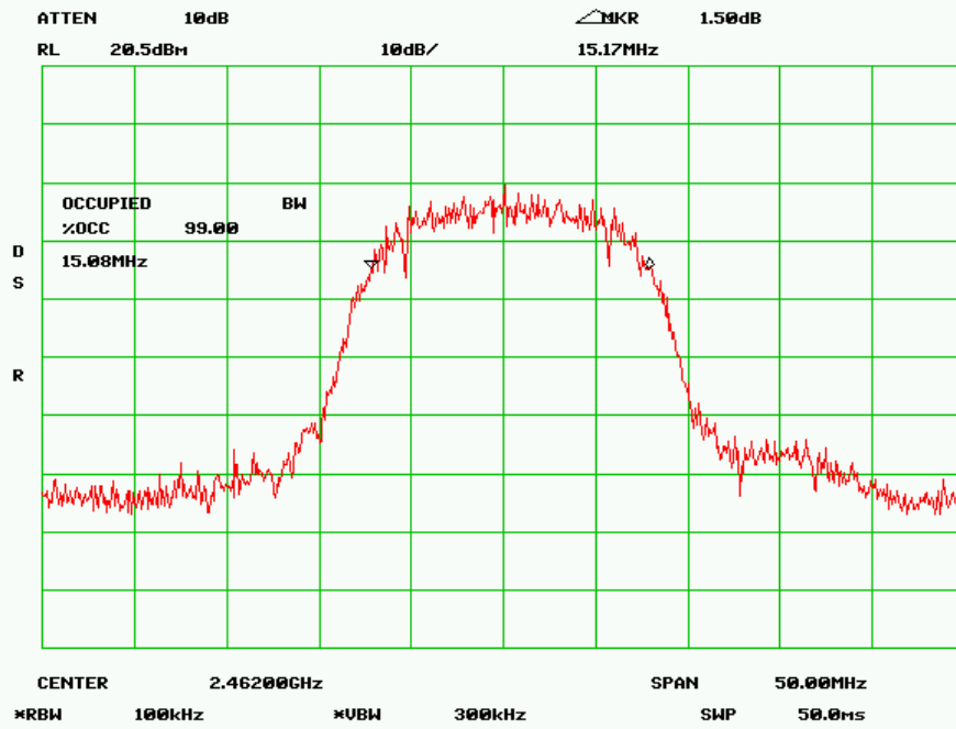
99% Bandwidth - High Channel (802.11b)
