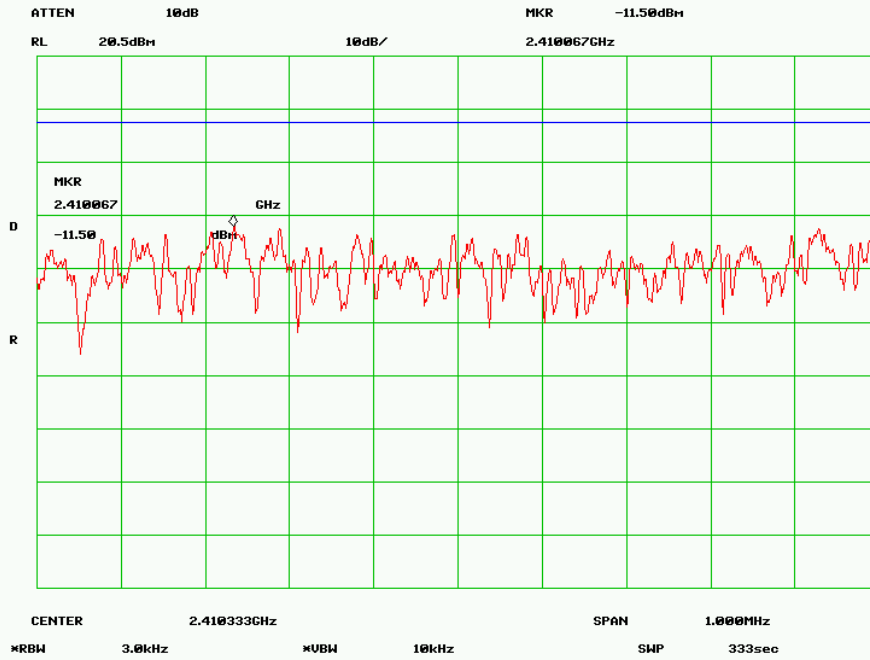
PSD Low Channel (802.11b)
