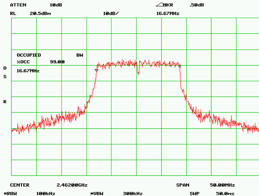
99% Bandwidth – High Channel (802.11g)
