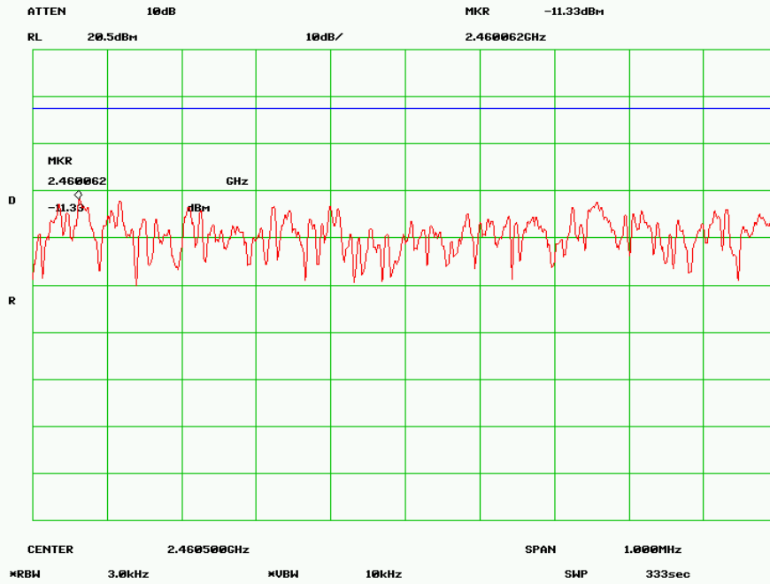
PSD High Channel (802.11b)
