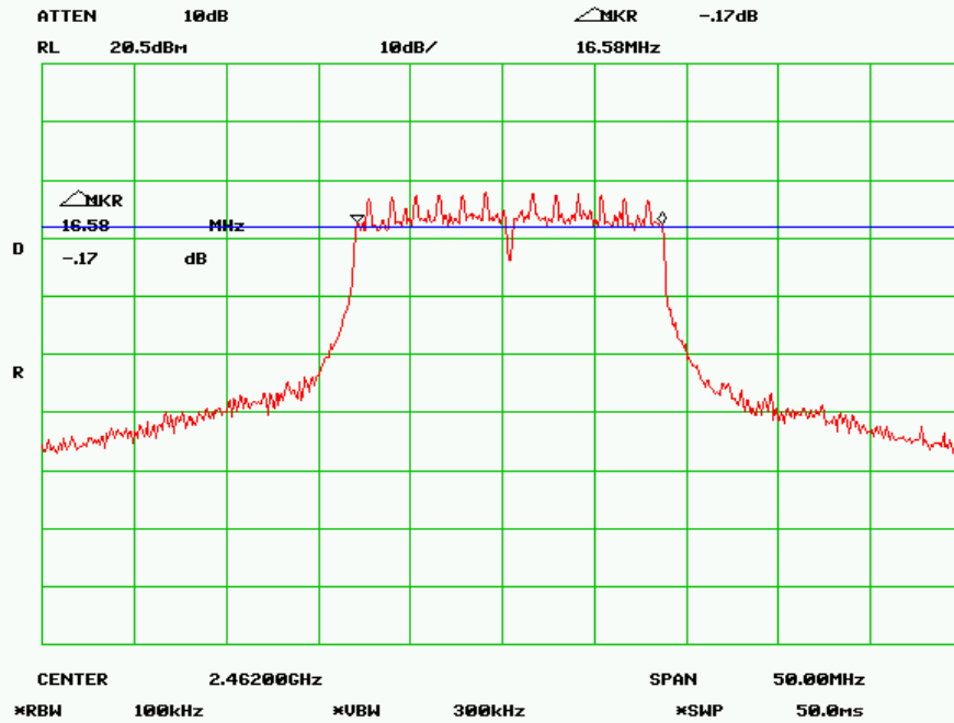
6 dB Bandwidth – High Channel (802.11g)
