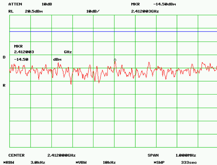
PSD Low Channel (802.11g)
