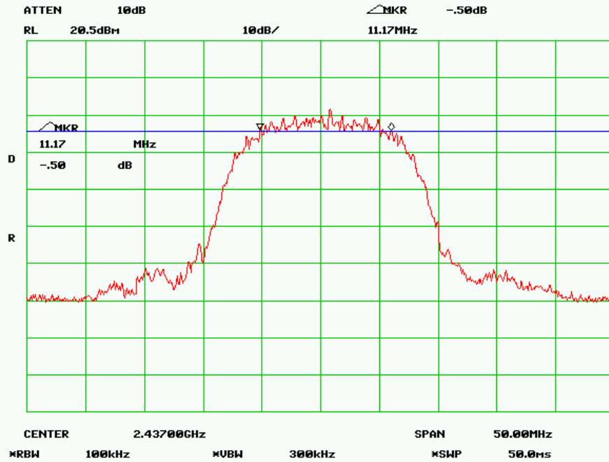
6 dB Bandwidth - Mid Channel (802.11b)
