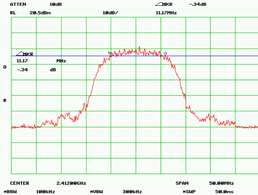
6 dB Bandwidth - Low Channel (802.11b)
