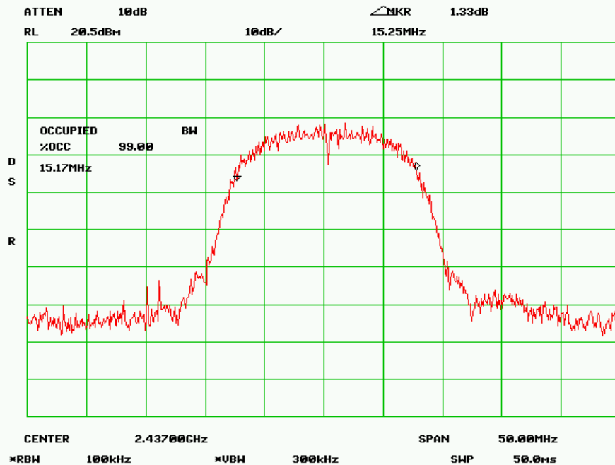
99% Bandwidth - Mid Channel (802.11b)
