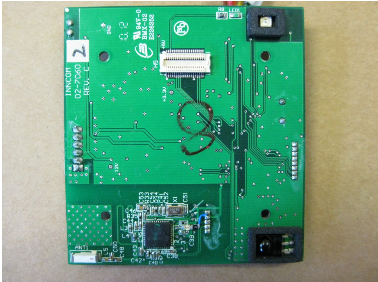
Backside of RF Board
