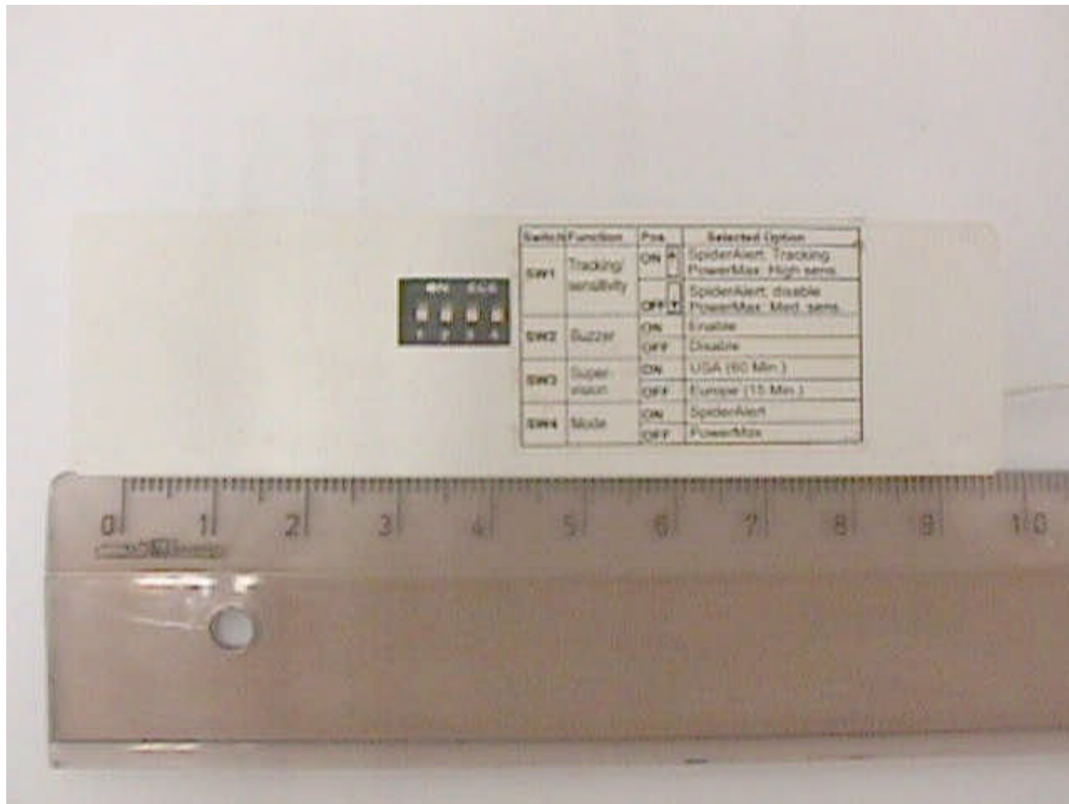
SPD-1000 bottom view
