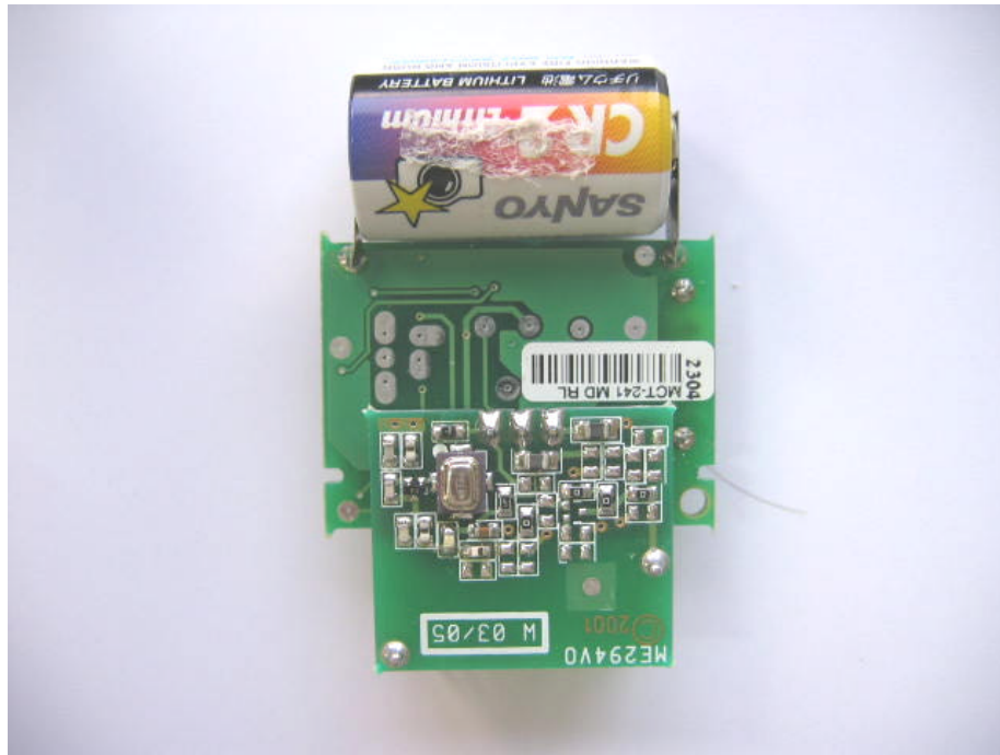
Photograph No.3 Pendant transmitter PCB assembly rear side
