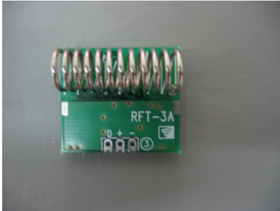
Photograph No.7 Pendant transmitter Print side of the RF PCB
