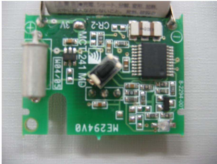
Photograph No.4 Pendant transmitter Component side of the main PCB
