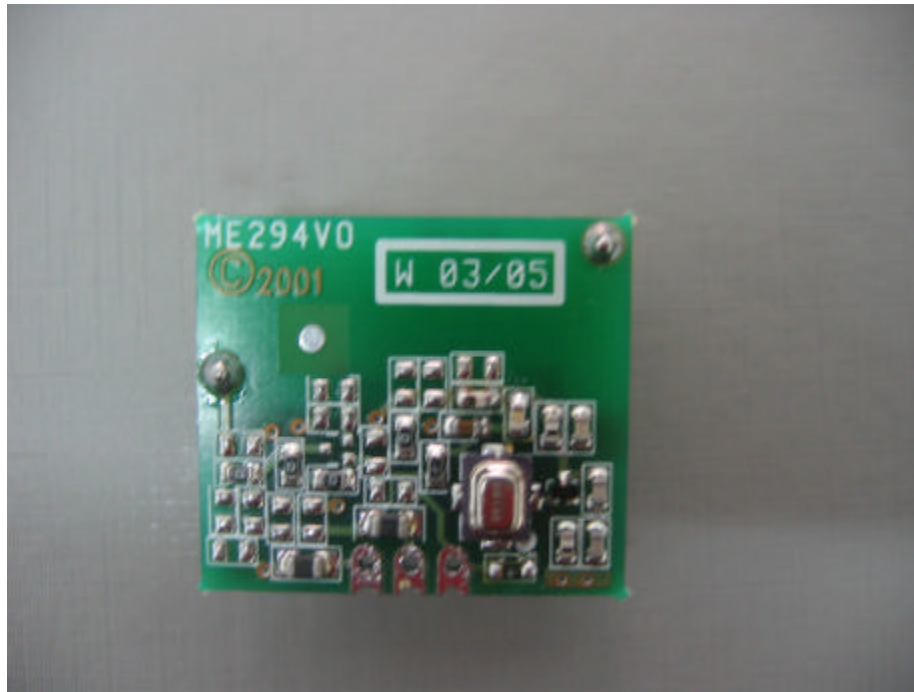
Photograph No.6 Pendant transmitter Component side of the RF PCB
