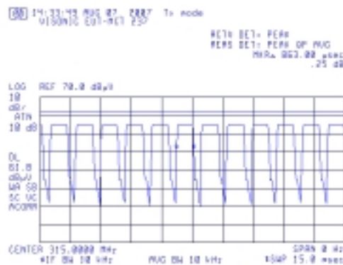
Plot # 10. Transmission duration - Tx on.
