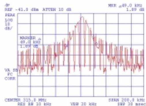
Plot # 14. 99% bandwidth test
