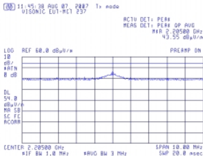
Plot # 6. The carrier frequency 7 th harmonic. Detector peak Test distance =3m.
