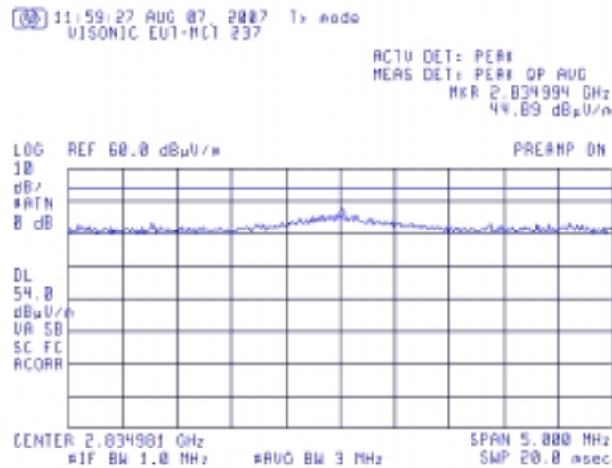
Plot # 7. The carrier frequency 9 th harmonic. Detector peak. Test distance =3m
