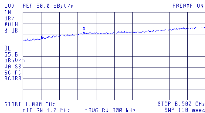
Plot # 3. Spurious emissions scan 1 – 6.5 GHz. Test distance =3m.
