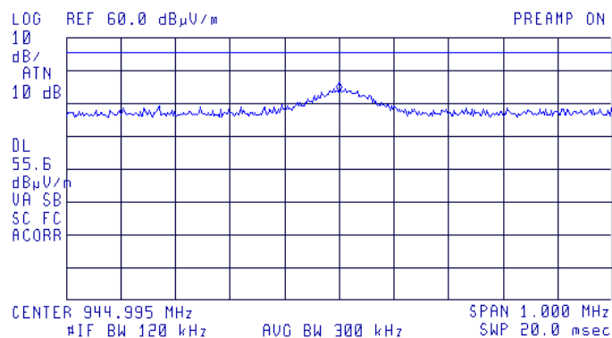
Plot # 4. The carrier frequency 3rd harmonic. Detector peak. Test distance =3m
