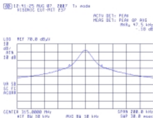
Plot # 13. 20 dB bandwidth test.
