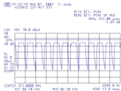
Plot # 11. Transmission duration - Tx off
