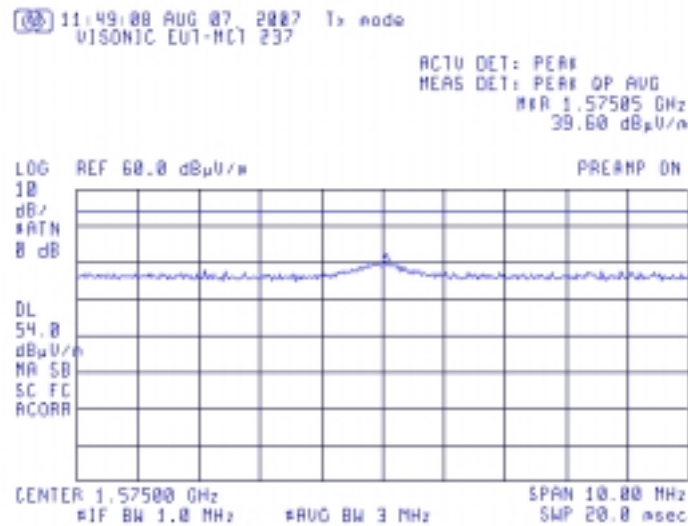
Plot # 5. The carrier frequency 5 th harmonic. Detector peak. Test distance =3m
