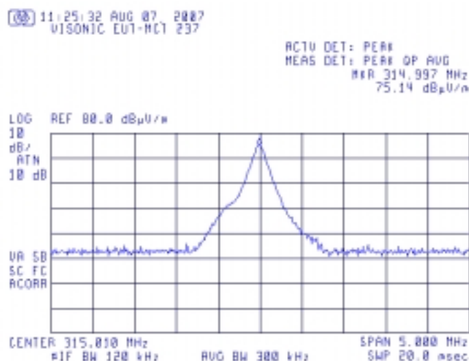
Plot # 1. Field strength of fundamental frequency 315 MHz.
