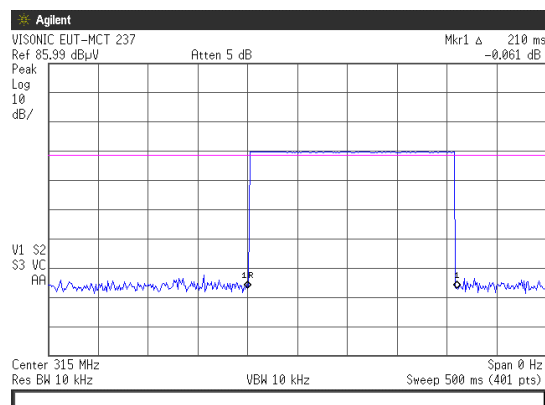
Plot # 12. Transmission message duration.
