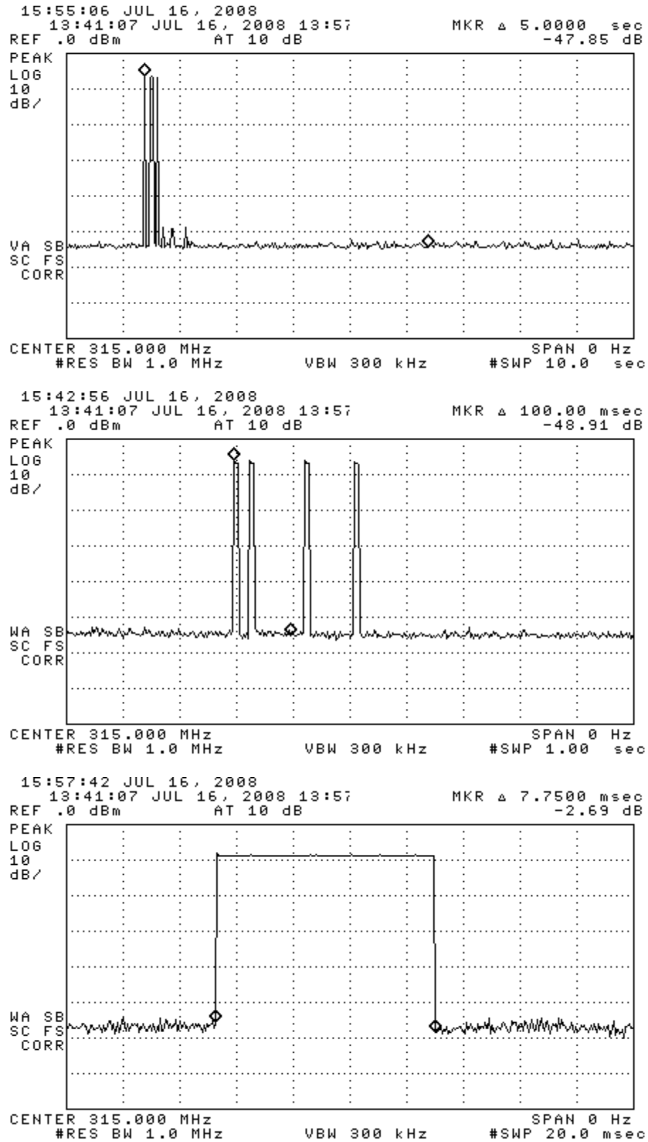
Figure 6.1. Transmissions modulation characteristics: (top) complete transmission after LF interrogation, (center) expanded transmission 4-words, (bottom) expanded word.
