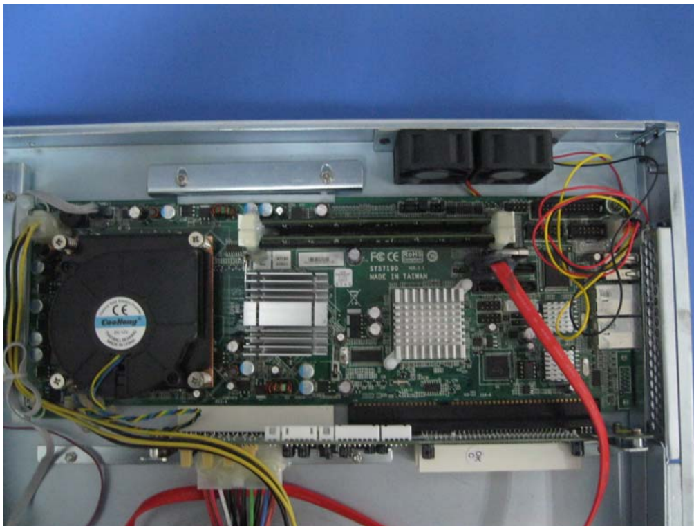
Mainboard Uncover View - 2
