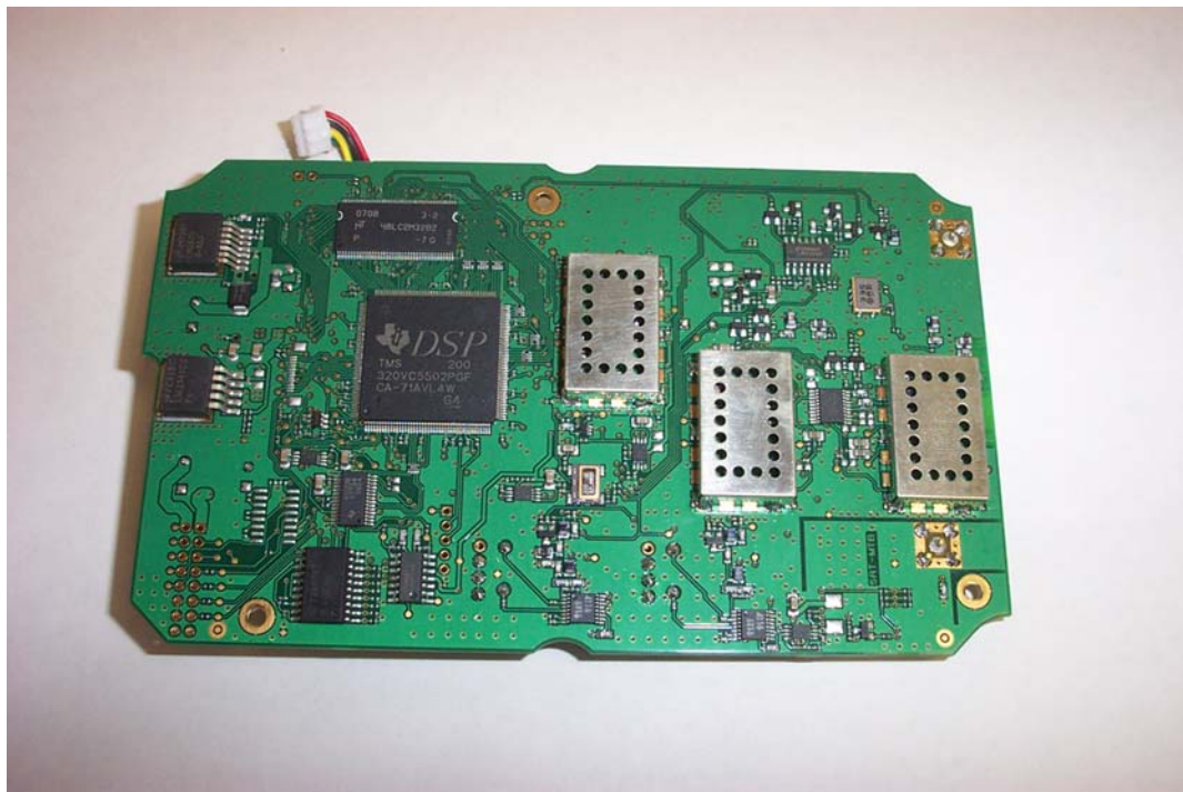
Figure 1: RF PCB; This is the SRT PCB licensed to Navico
