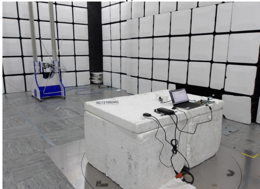
Photo 1.5-4 – Back View of the Test Setup, 3m - Out of band emissions 30 - 1000MHz
