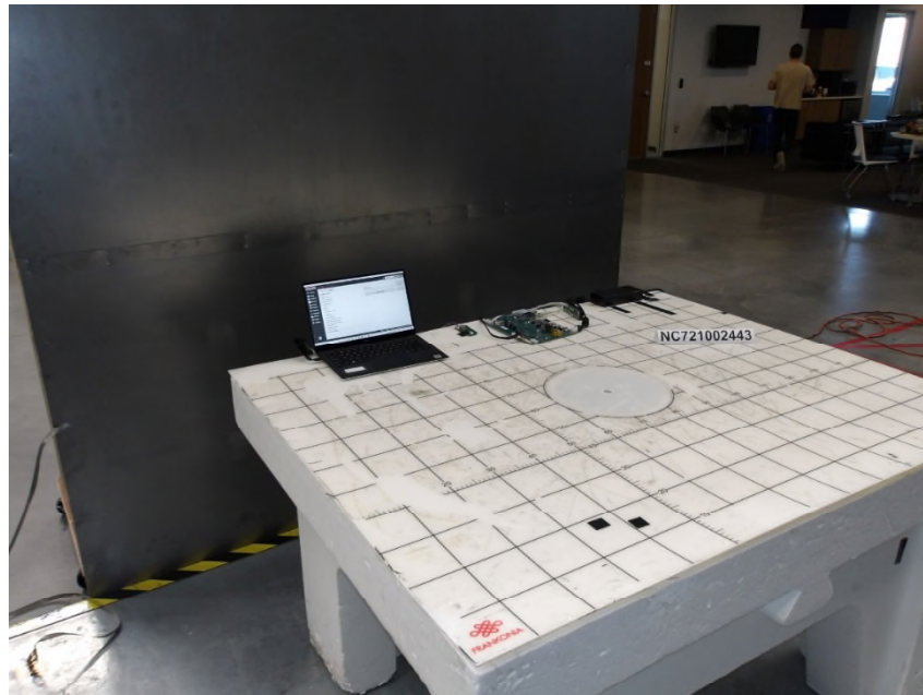
Photo 1.2-1 – Conducted Emission Test Setup [Front View]
