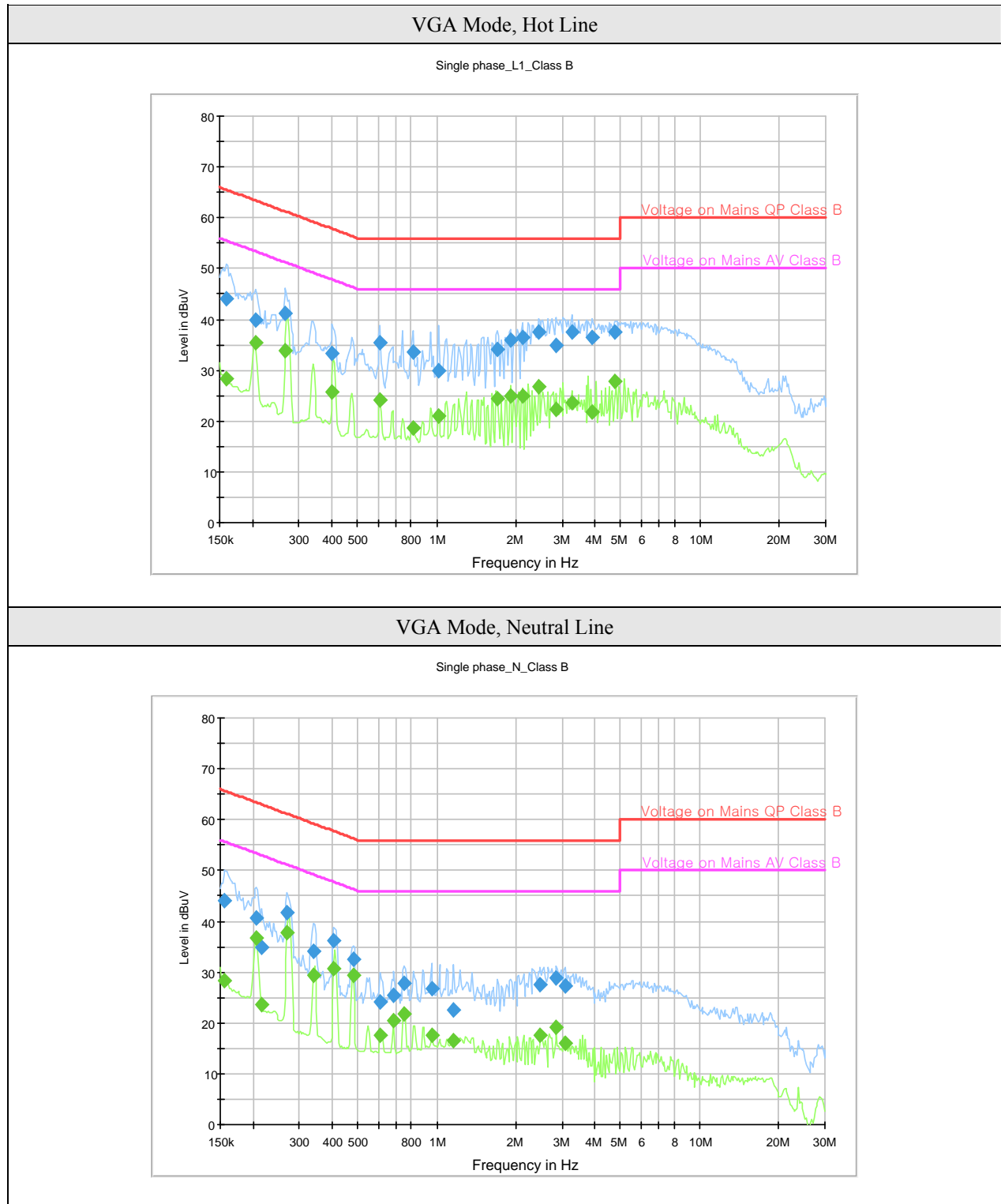
Figure 3. Graphical representation of conducted emissions, VGA Mode
