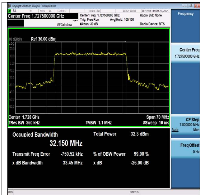
NTNV-n66-PC3-15-35-L-DFT-BPSK-Outter_Full-Ant1- PASS
