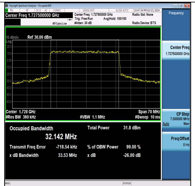
NTNV-n66-PC3-15-35-L-DFT-QPSK-Outter_Full-Ant1- PASS
