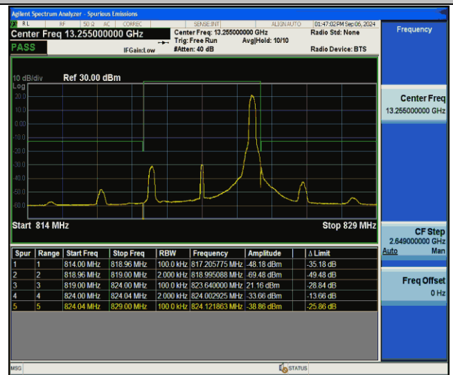
26(814-824)-5MHz-QPSK-26765-1RB#24-PASS
