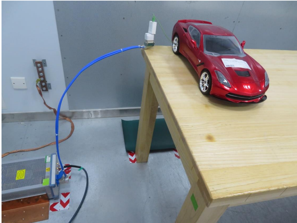
Conducted Emissions test setup photo
