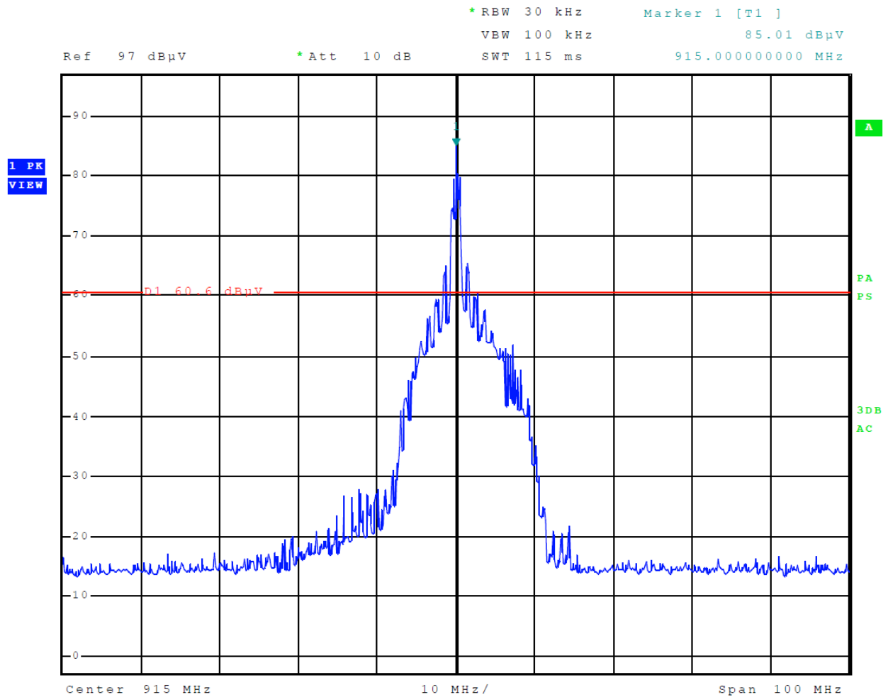
Figure 4 Emissions Mask
