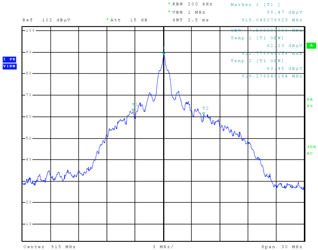
Figure 2 Occupied Bandwidth
