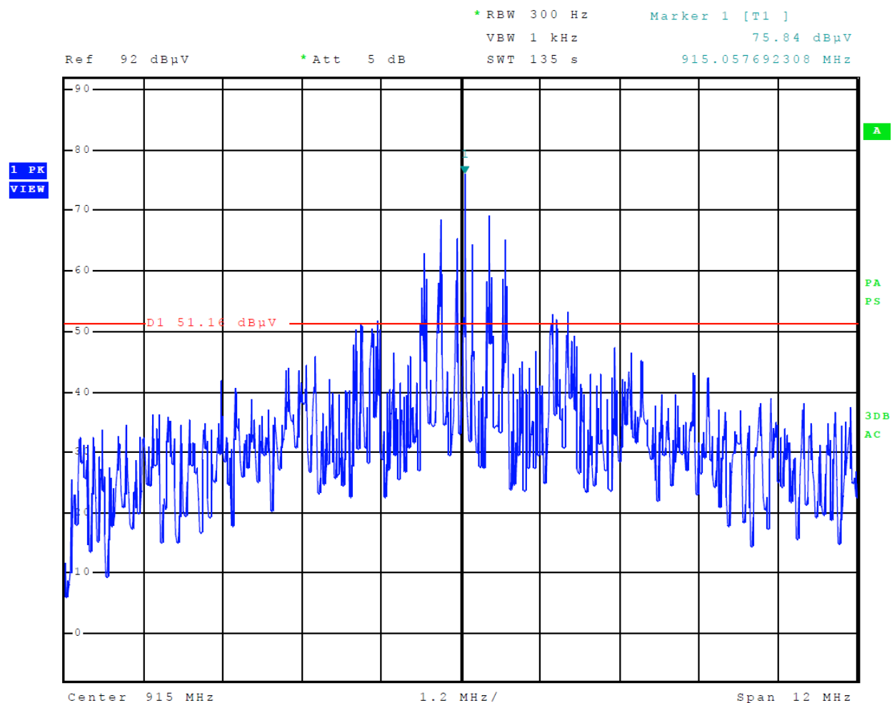
Figure 3 Emissions Mask
